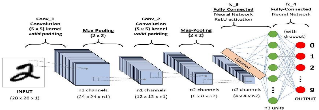
Fig 2 Connectivity of the Pooling and Kernels in CNN
