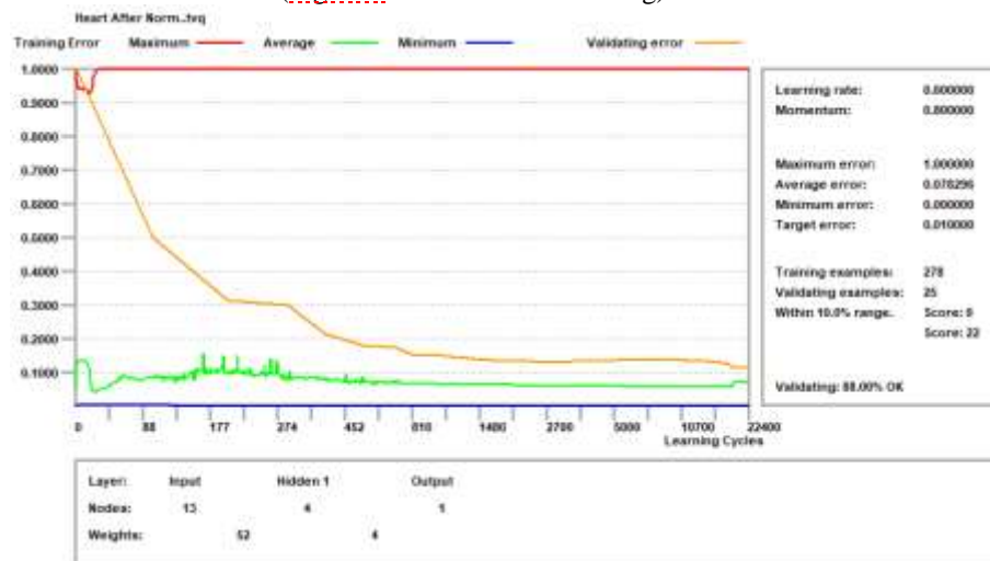
(Figure 4: History of training and validation)
