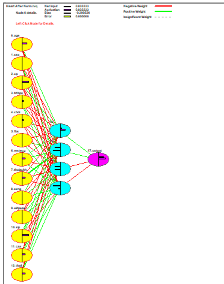
(Figure 1: Architecture of the proposed model)
