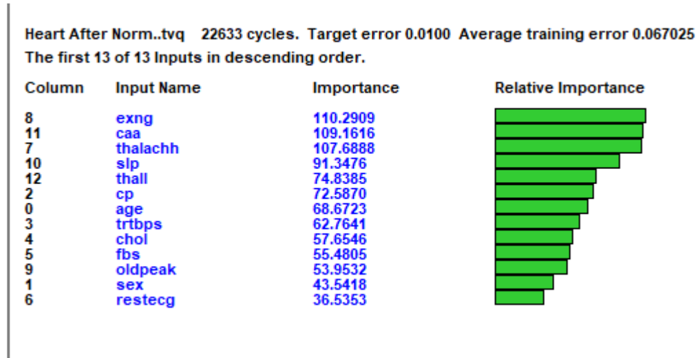
(Figure 2: Features importance)
