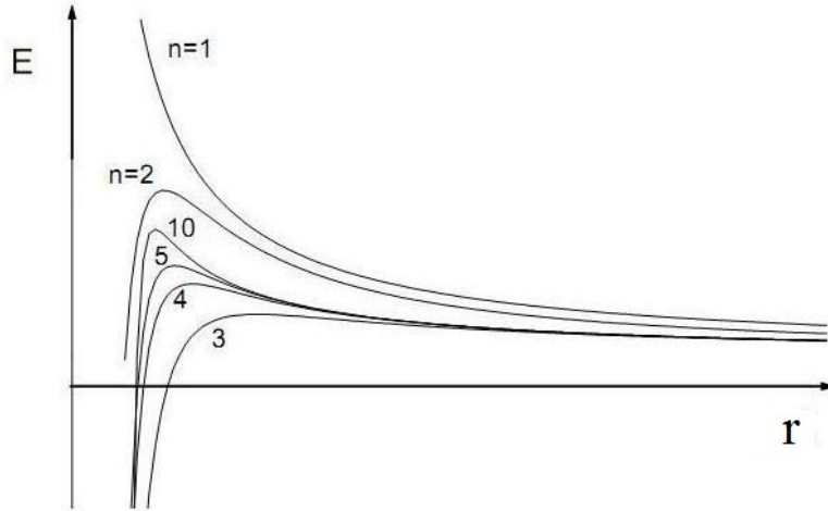
Figure 6: Graphs of functions E(r) in n -dimensional spaces
