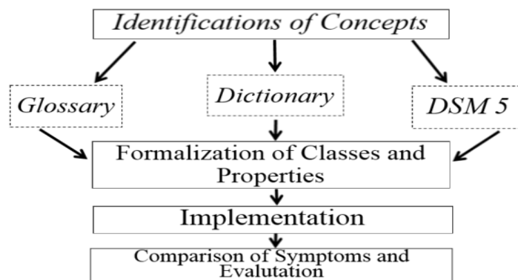
Fig. 1. The process of building a DSM-5 compliant ontology.
