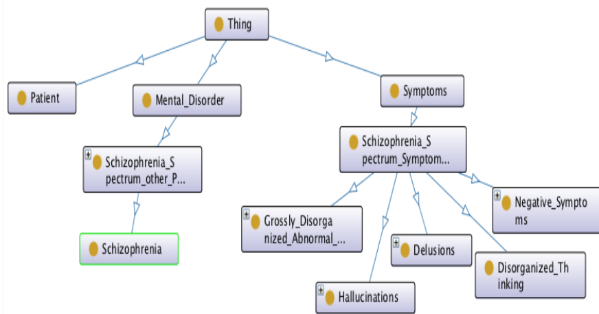
Fig. 2. Top Level of the Schizophrenia Spectrum Ontology.
