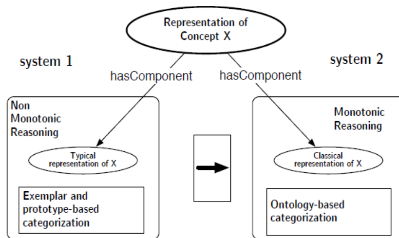
Fig. 3. The conceptual architecture we propose.
