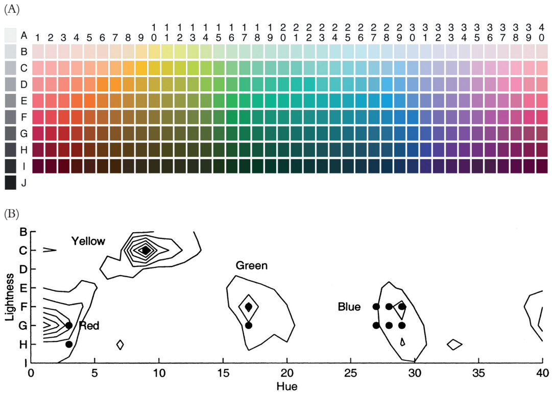
Figure 28.1 (A) Munsell colour palette and (B) contour plot of WCS best-example choices compared with best examples of English colour terms for the chromatic Hering primaries.
