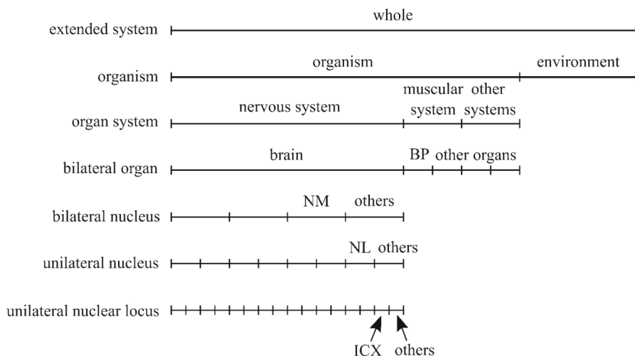
Fig. 6 A partition of the anatomical organisation of the barn owl down to 7 levels of anatomy. The highest level is trivial (it partitions the whole system into itself) and the lowest level could be indefinitely refined by further partitions
