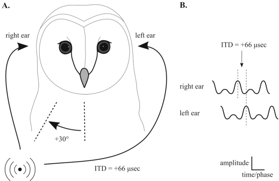
Fig. 2 A Sound waves from sources at, e.g., +30^\circ reach the left ear 66 \mu\text{sec} after the right ear. B The interaural (between-ears) time delay (ITD) is encoded by the delay in the propagation of the sound waves through the owl's left and right ears. Note that amplitude is on the y-axis and time (or phase) is on the x-axis
