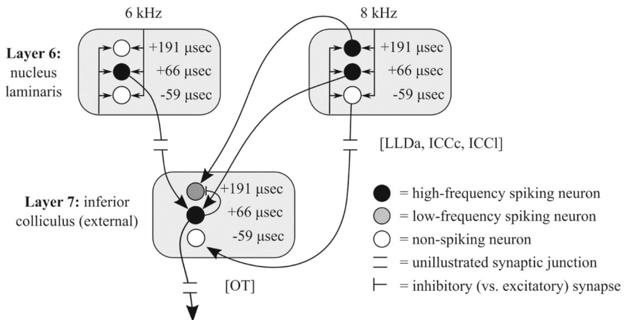
Fig. 5 The ICX receives the true IPD signal (e.g., 66 μs) across all frequency channels and phantom IPD signals (e.g., 191 μs) in specific frequency channels (e.g., 8 kHz). It uses lateral inhibition between frequency channels to single out the strongest signal: the true IPD signal will overpower, inhibit, and silence the phantom IPD signals. Then the ICX delivers the mode-ITD signal to the optic tectum (OT)
