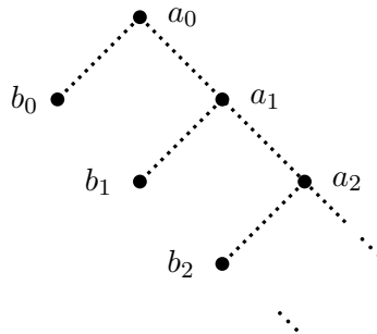
Figure 3. Model \mathcal{M}_2
