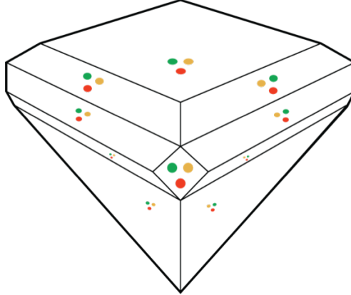
Figure 1: Diamond \mathcal{D} with geometric point \mathrm{Spa} C \rightarrow \mathcal{D} pulled back through a quasi-pro-étale cover X \rightarrow \mathcal{D} , resulting in profinitely many copies of \mathrm{Spa} C [16].
