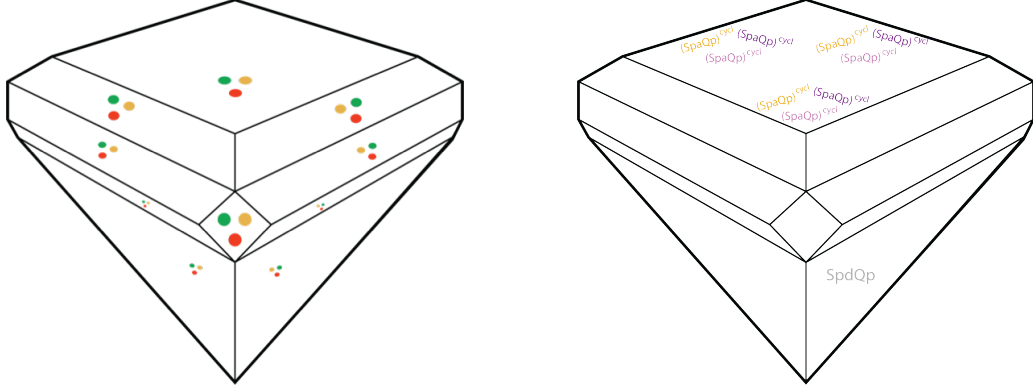
Figure 3: Diamond SpdQ_p = Spa(Q_p^{cycl}) / \underline{Z_p^\times} with geometric point Spa C \rightarrow \mathcal{D}
