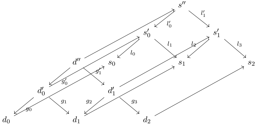
Figure 8: Pro-diamond in \mathcal{D}^{\infty} and Pro-Emergence in S
