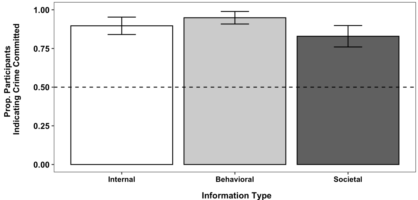
Fig. 3. Proportion of participants indicating that a given individual was incarcerated because he committed a crime, Study 2b. Error bars represent 95% confidence intervals.
