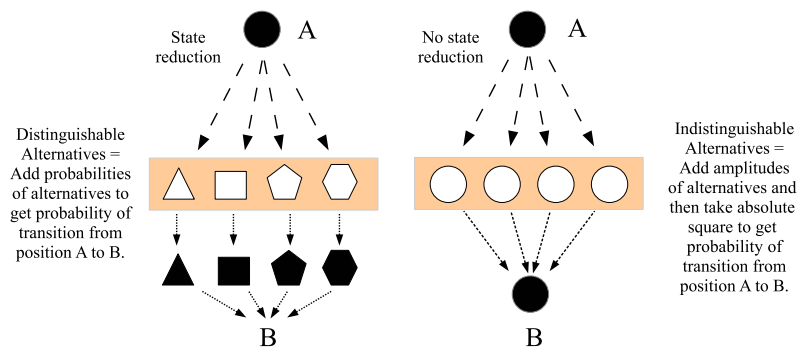
Figure 15. Grating metaphor illustrating the Feynman rule.
