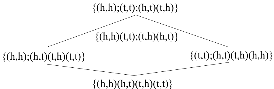
Figure 14: Lattice of possible mixed and pure boson states (two particles and two particle states)
