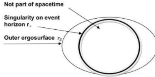
Figure 4. Rotating gravitational singularity with singular support on outer ergosurface
