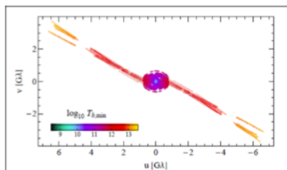
Figure 2. Fourier coverage (uv-coverage) of the fringe fitted data (i.e., reliable fringe detections) of the Radio Astron observations of BL Lac on 2013 November 10-11 at 22 GHz. Color marks the lower limit of observed brightness temperature obtained from visibility amplitudes. Adopted from [19]
