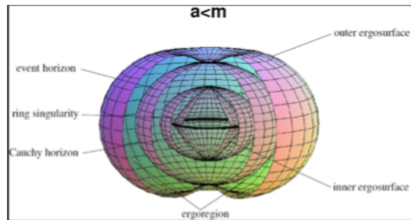
Figure 3. Ergosurface, horizon, and singularity for slow Kerr black hole
