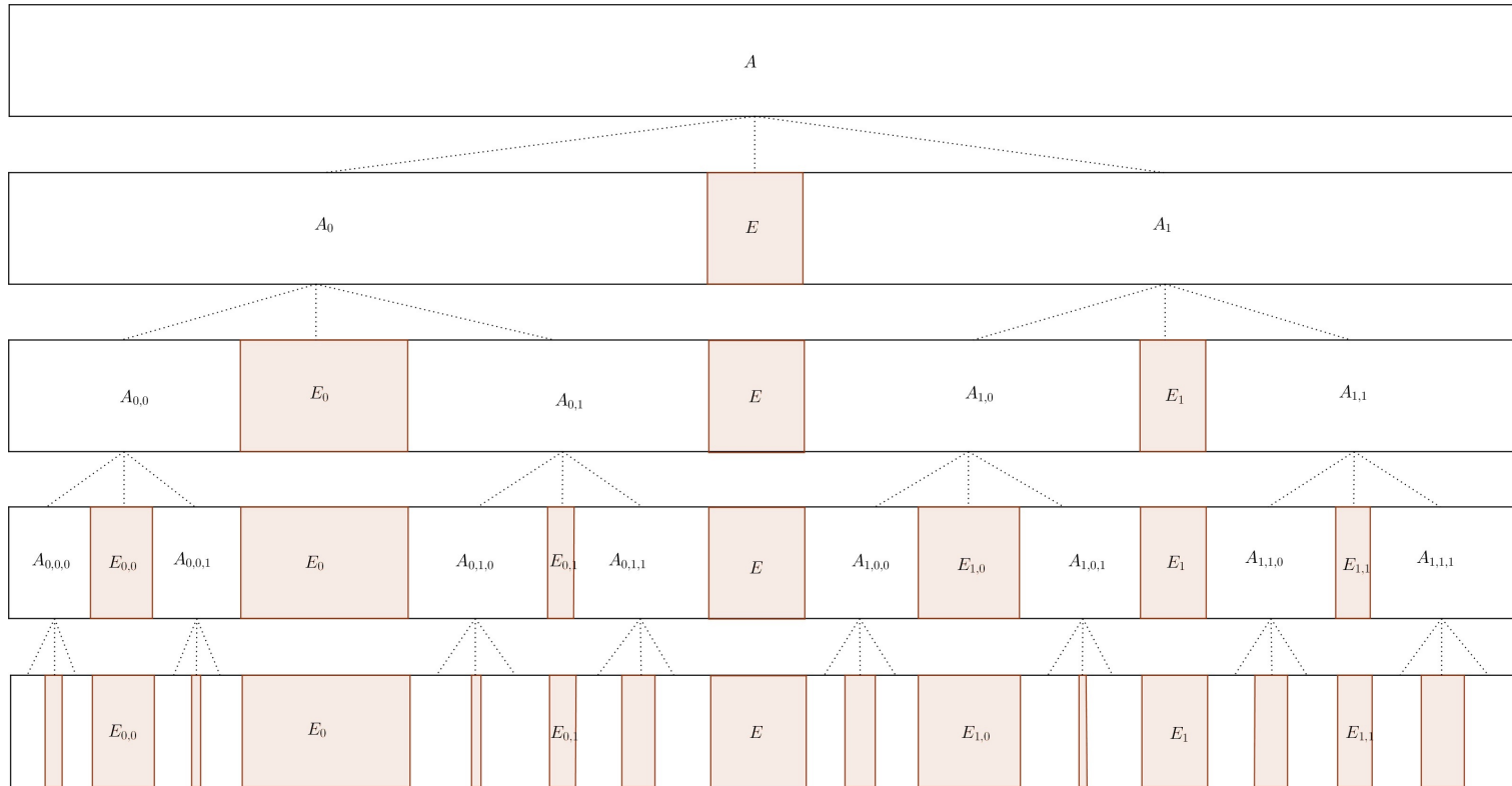
Figure 3.2: A tripartition tree \mathcal{T} of A
