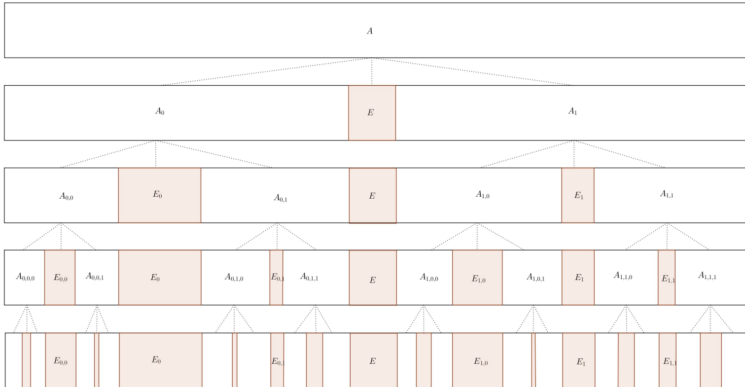
Figure 2: A tripartition tree \mathcal{T} of A
