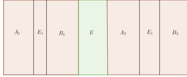
Figure 3: Claim in the proof of Theorem 19
