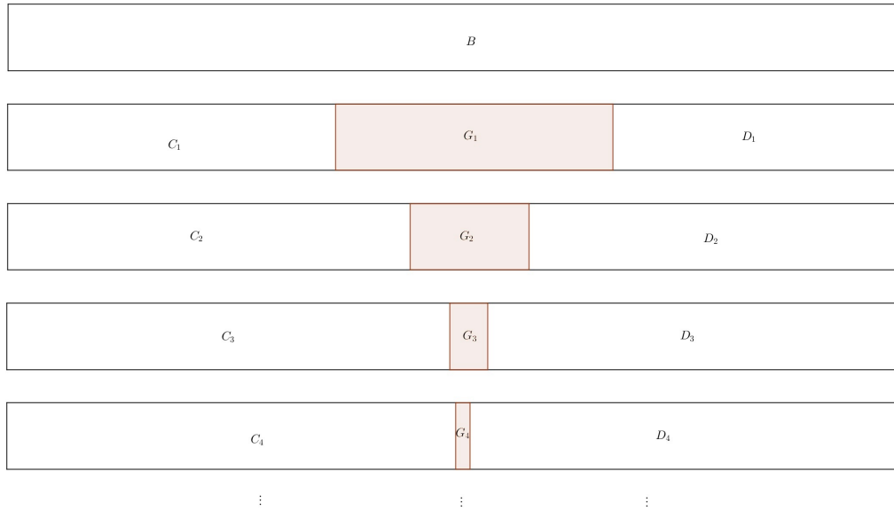
Figure 1: Savage's error reducing partitions
