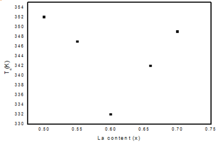
Fig. (5): Variation of Curie temperature with La content (x) for the nanocrystalline samples \text{La}_x\text{Sr}_{1-x}\text{MnO}_3
