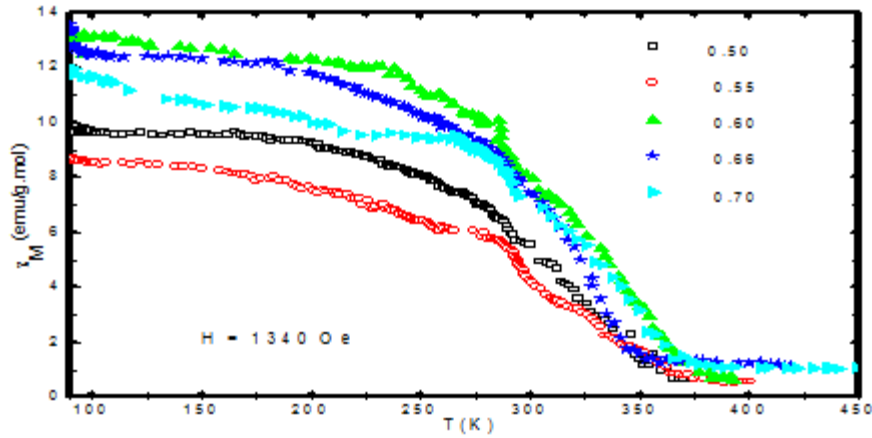
Fig.(4a): Dependence of molar magnetic susceptibility on absolute temperature for the nanocrystalline samples \text{La}_x\text{Sr}_{1-x}\text{MnO}_3 0.50 \leq x \leq 0.70 .
