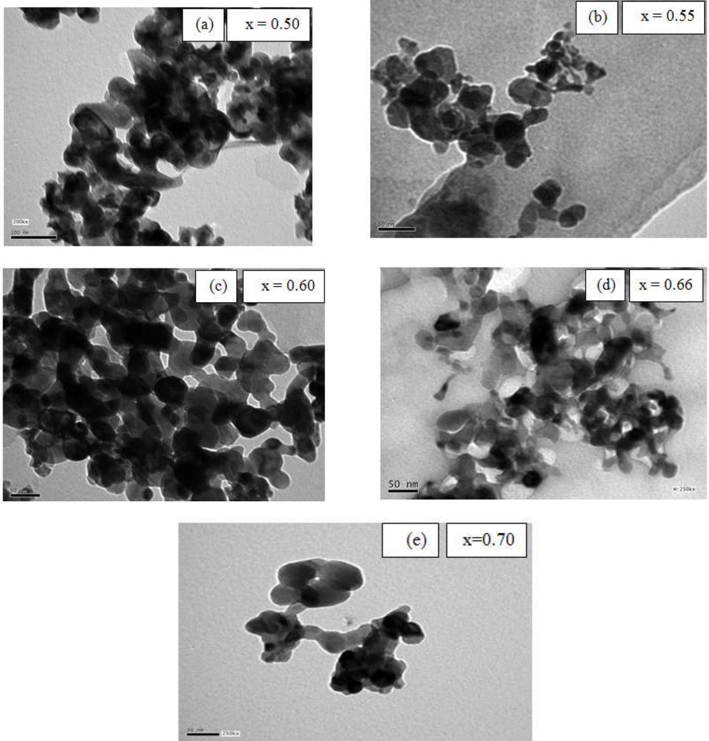
Fig. (3: a - e) TEM micrographs of the nanocrystalline samples \text{La}_x\text{Sr}_{1-x}\text{MnO}_3 where 0.50 \leq x \leq 0.70 .
