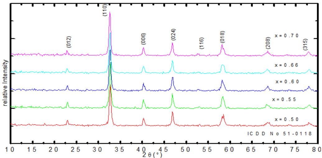
Fig. (1): X-Ray Diffraction (XRD) patterns of the samples La_xSr_{1-x}MnO_3 ; 0.50 \leq x \leq 0.70 .
