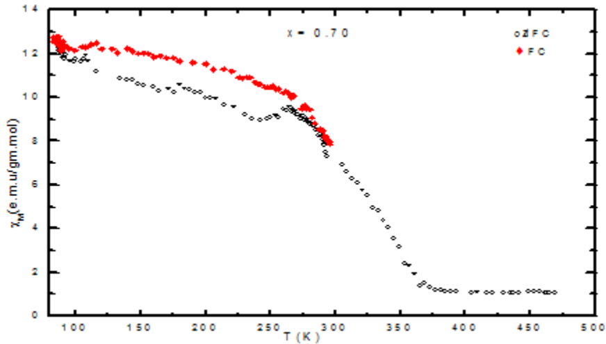
Fig.(4a): Dependence of molar magnetic susceptibility on absolute temperature for the nanocrystalline samples \text{La}_x\text{Sr}_{1-x}\text{MnO}_3 0.50 \leq x \leq 0.70 .
