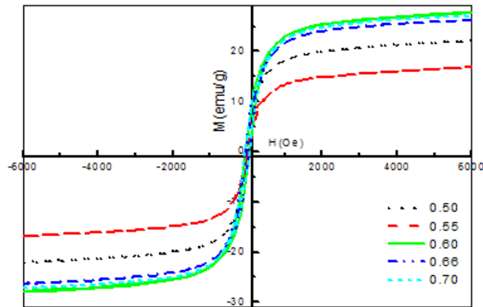
Fig. (6): Magnetic hysteresis of all nanocrystalline samples \text{La}_x\text{Sr}_{1-x}\text{MnO}_3 ; 0.50 \leq x \leq 0.70 .
