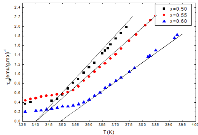
Fig. (7) Change of the reciprocal of molar susceptibility with absolute temperature for nanocrystalline samples \text{La}_x\text{Sr}_{1-x}\text{MnO}_3
