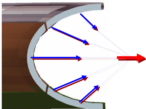
(VI-i-2~12) Symmetric Activation section of front PNT activator
