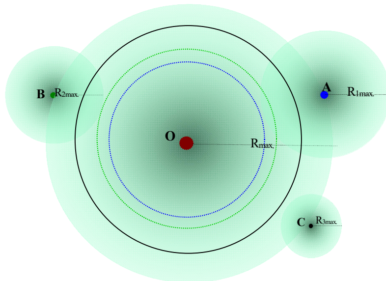
(V-iv-5-c) General relative layout of “peripheral inexpedient assimilable globose field lamella”
