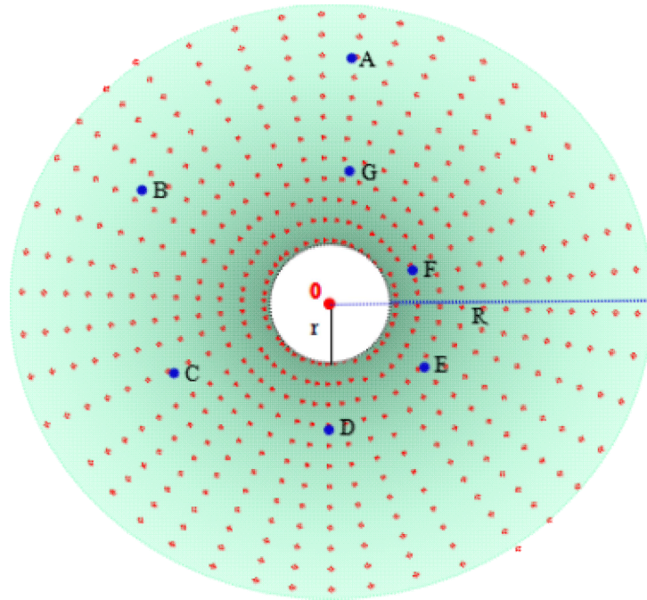
(IV-ii-7) Analytic illustration of observation view discrepancy of the Big Bang of cosmos in different observation position
