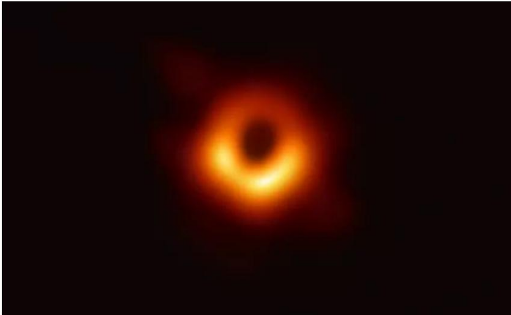
(VII-iii-3) The picture above come from a paper named “strangeness of Black Hole” which I encountered in researchgate.net website by chance in Oct. 2020.
