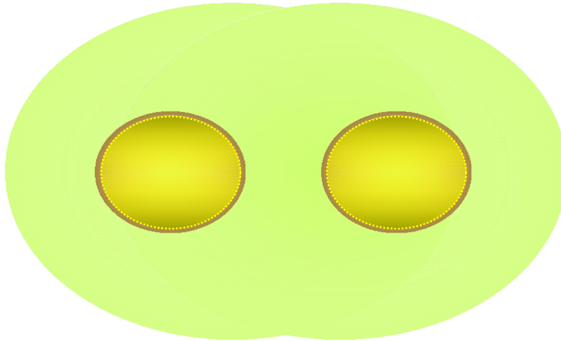
(IV-ii-2) Double-yolk egg model configuration & overall arrangement of homogenous cosmos
