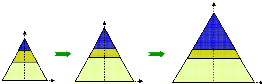
(IV-i-7) Quantitative change of the third stage of cosmic evolution in expansion increase model of parallel cone
