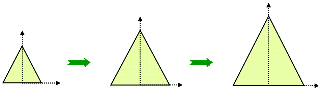
(IV-i-5) Quantitative change of space field development in expansion increase model of parallel cone
