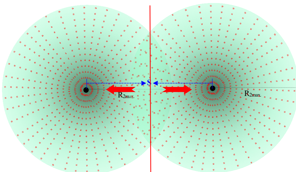
(III-i-4-e) Electromagnetic repulsion between negative electric field and negative electric field
