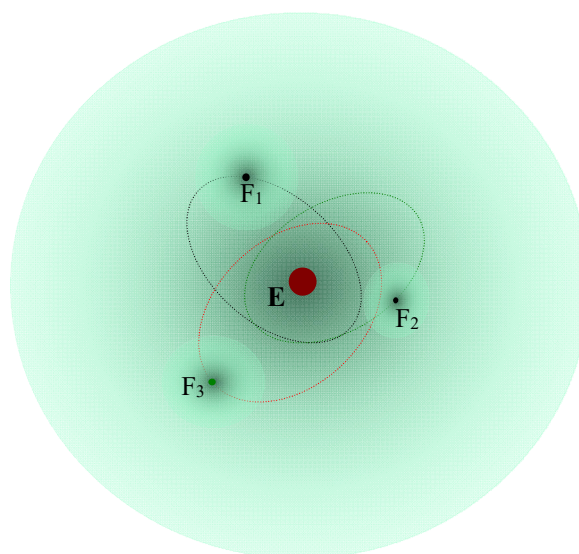
(V-iv-5-e) Galaxy among celestial bodies under reciprocity of positive gravity
