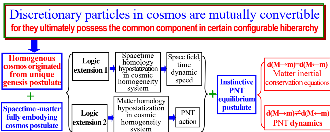
(II-i-3) Simplified logic constitution of Homogenous Cosmos Originated from Unique Genesis
