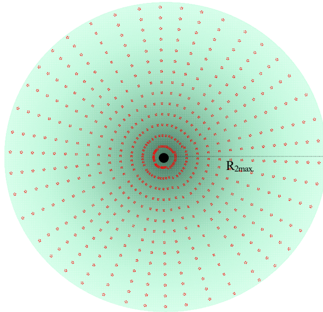
(III-i-4-b) Negative electric field with genic preponderance
