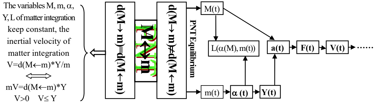
(II-i-1) logic constitution of PNT dynamics
