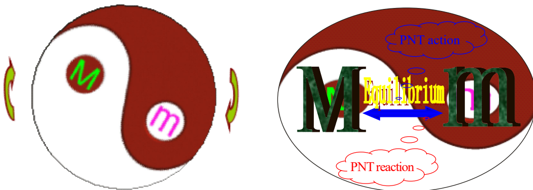
(G-ii-3) Instinctive PNT equilibrium icon
