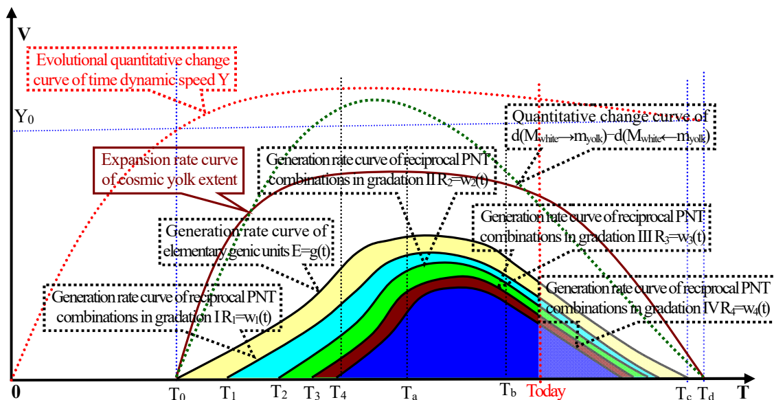
(IV-iv-3) Quantitative change rate curve of extent expansion of cosmic yolk extent, quantitative change curve of acclimatization cushion of time dynamic speed of cosmic yolk extent, quantitative change rate curve of aberrant convergence of cosmic esse due to PNT reciprocal gelation under cosmic live input of d(M_{white} \rightarrow m_{yolk}) > d(M_{white} \leftarrow m_{yolk})
