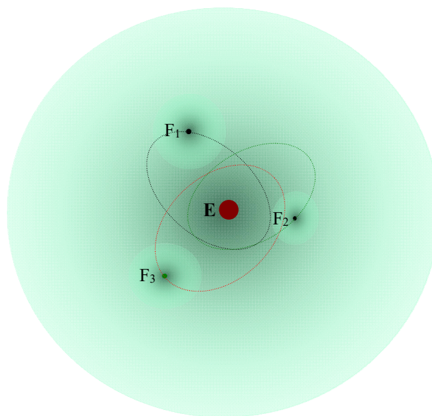
(III-i-2-h) Small celestial bodies go around big celestial body as planets for proper gravitational reciprocity.
