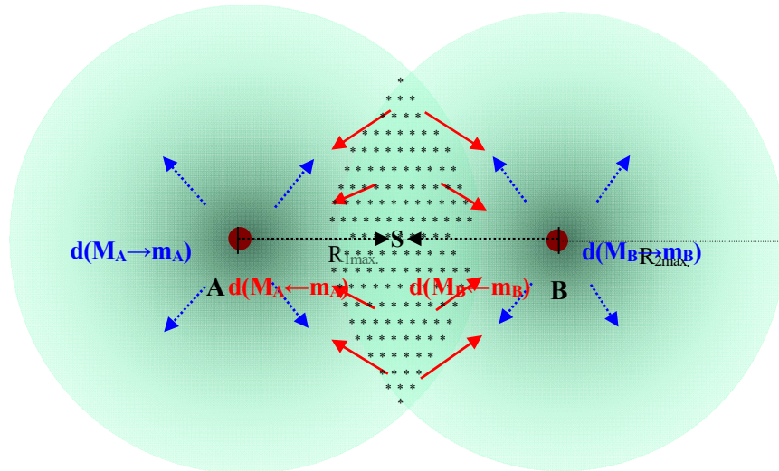
(V-iv-5-b) Reciprocity model of gravity due to [matter field superposition disturbance + (PNT action + Instinctive PNT equilibrium)]
