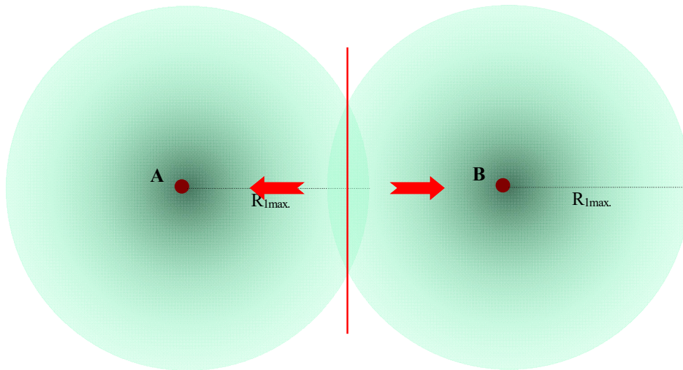
(III-i-2-i) The opposing gravitation reciprocity between two celestial bodies in equivalent mass scale
