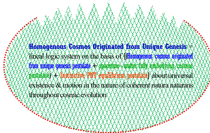
(VII-i-1) Illustration of distinctive geometrical aggregation of Homogenous Cosmos Originated from Unique Genesis
