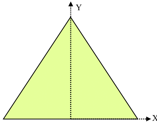
(IV-i-4) Quantitative change of cosmic evolutionary multiplication in expansion increase model of parallel core
