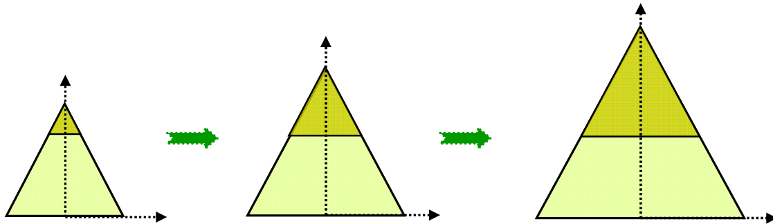
(IV-i-6) Quantitative change of the second stage of cosmic evolution in expansion increase model of parallel cone
