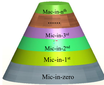
(1) Taper distribution pattern of spacetime momentum delamination hoarding of reciprocal PNT combination in n configurable hiberarchies
