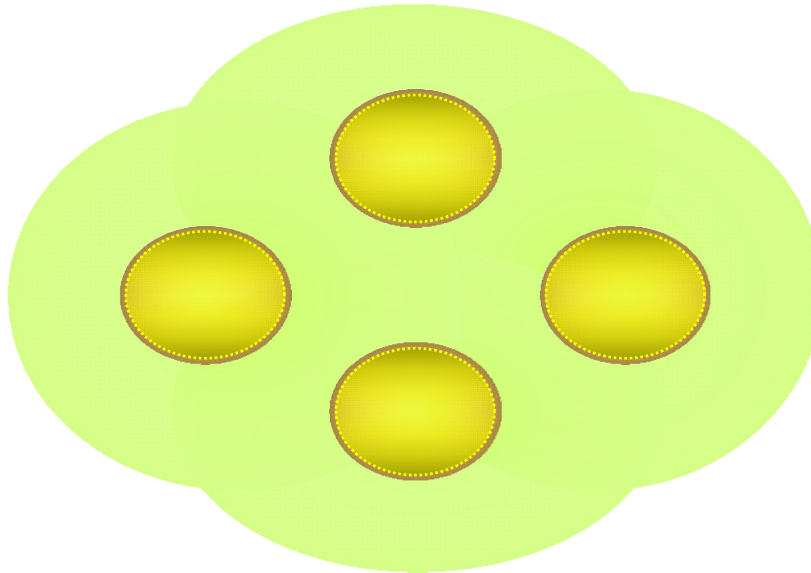
(IV-ii-3) Multi-yolk egg model configuration & overall arrangement of homogenous cosmos
