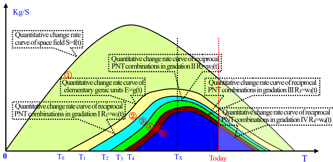
(IV-i-9) Integrated quantitative change rate curve of sequential homologous cosmogony through and through
