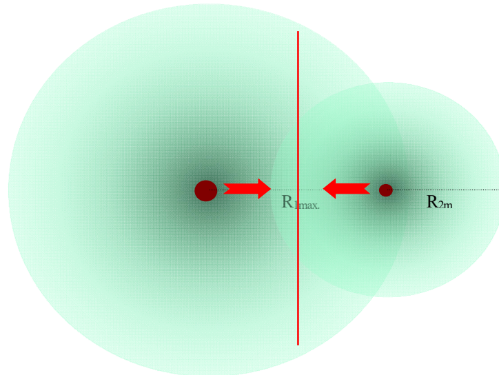
(V-iv-5-d) Mass disparity accessible to positive gravity
