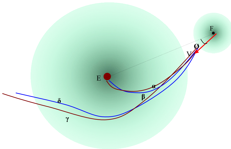
(III-i-2-g) Gravitational motion track contrast of object moving in accordance with gravitational reciprocity of Homogenous Cosmos Originated from Unique Genesis and in accordance with gravitational reciprocity of tradition, whose initial momentum is enough to break through the peripheral inexpedient assimilable globose field lamella
