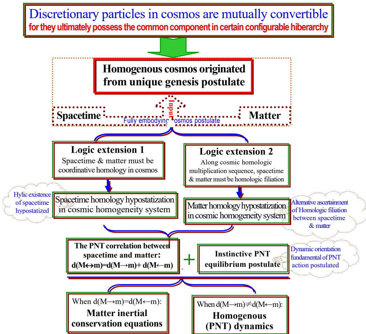
(G-ii-1) Inborn logic constitution of PNT dynamics
