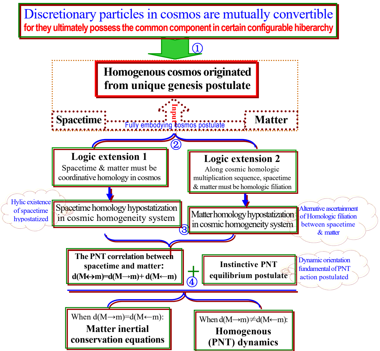
(II-i-2) Inborn logic constitution of PNT dynamics
