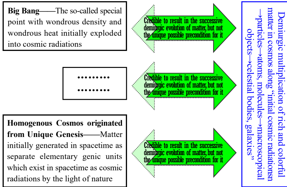
(IV-iv-4) Amphibolous demonstration correlation between “cosmic background radiation” and “Big Bang”
