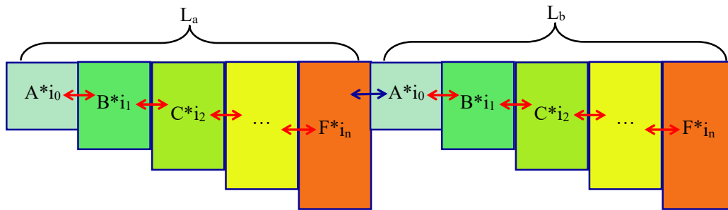
(V-iv-2-b) Connatural linear connection & succession among optimum PNT genic linkages in space field
