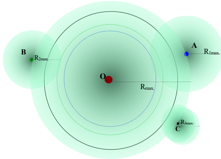
(III-i-2-e) General relative layout of “peripheral inexpedient assimilable globose field lamella” and “central expediently assimilable globose field extent” for gravitational reciprocity
