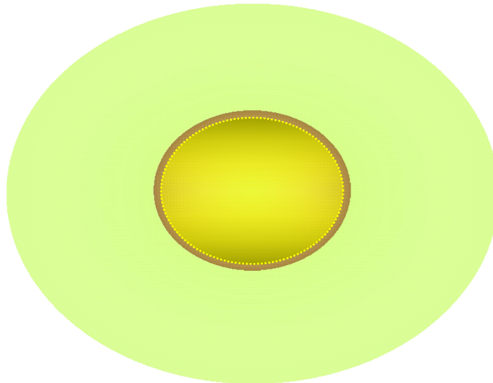
(IV-ii-1) Egg model configuration & overall arrangement of homogenous cosmos
