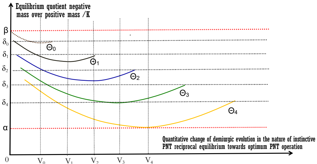
(IV-i-3) Distribution of “equilibrium quotient negative mass over positive mass” K of matter integration along quantitative change of demiurgic evolution in the nature of instinctive PNT reciprocal equilibrium towards optimum PNT operation
