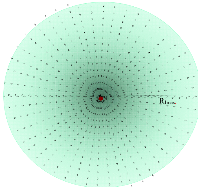
(III-i-4-a) Positive electric field with genic insufficiency
