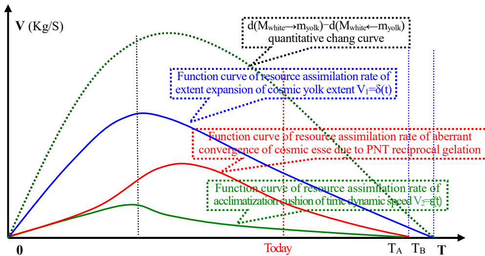
(IV-ii-4) Contrast illustration of function curve of resource assimilation rate of extent expansion of cosmic yolk extent, function curve of resource assimilation rate of acclimatization cushion of time dynamic speed and function curve of resource assimilation rate of aberrant convergence of cosmic esse due to PNT reciprocal gelation.
