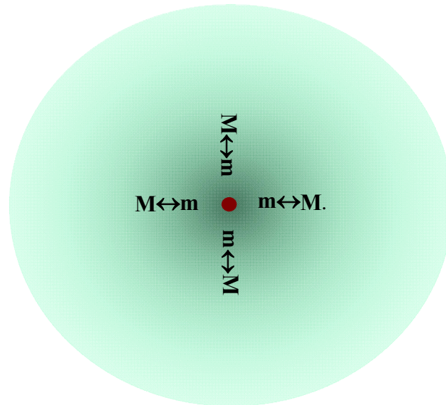
(II-i-1-a) Configuration and overall arrangement of matter integration
