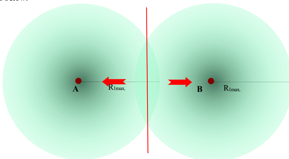
(V-iv-5-f) Mass approximation accessible to negative gravity
