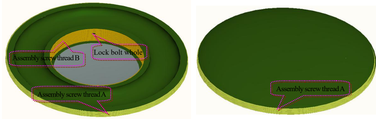
(VI-i-2~63) Inner view of tyre core lower jacket plate
