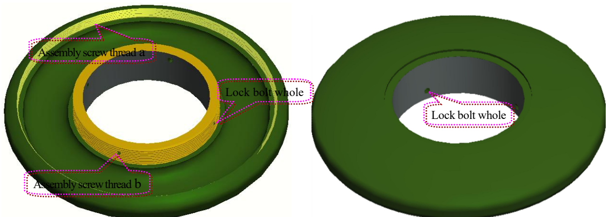
(VI-i-2~66) Inner view of tyre core upper jacket plate
