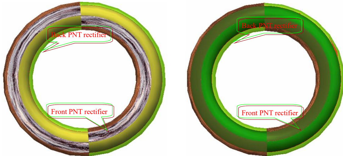
(VI-i-2~21) Upper limb view of ‘PNT rectifiers + tyre core’
