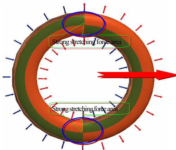
(VI-i-2~16) Integrate stimulation status of tyre core in PNT activation model of front “ \phi angle two-dimensional symmetric activation” + back “ \phi angle three-dimensional symmetric activation”
