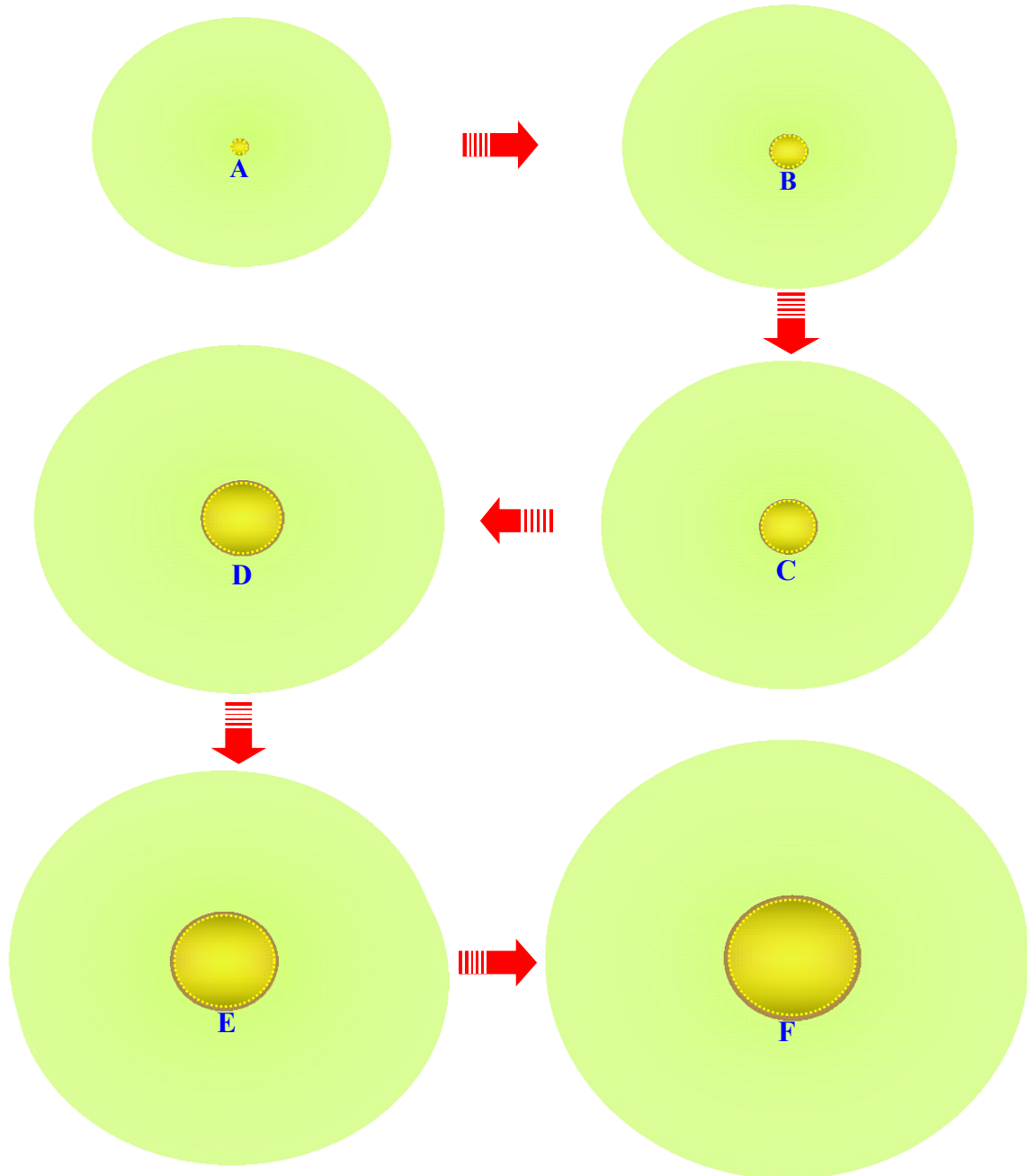
(IV-ii-6) integrative extent expansion of cosmic yolk extent following quantitative change of bidirectional lineal homologic pervasion of d(M_{white \rightarrow m_{yolk}}) > d(M_{white \leftarrow m_{yolk}})
