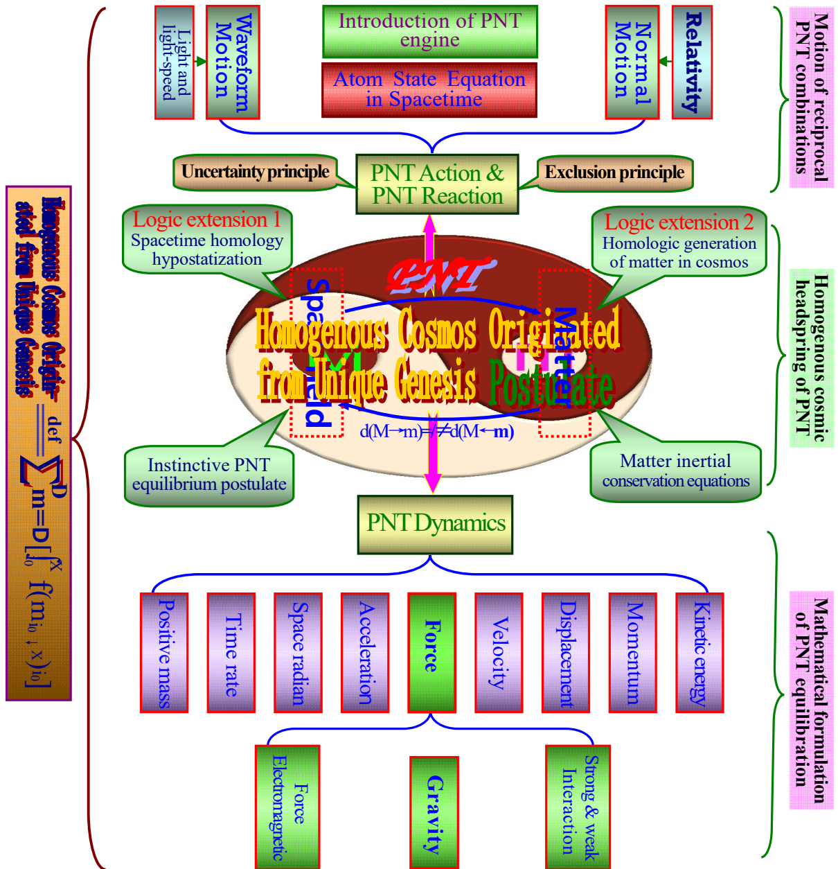
(G-ii-2) Integrative logic constitution of Homogenous Cosmos Originated from Unique Genesis
