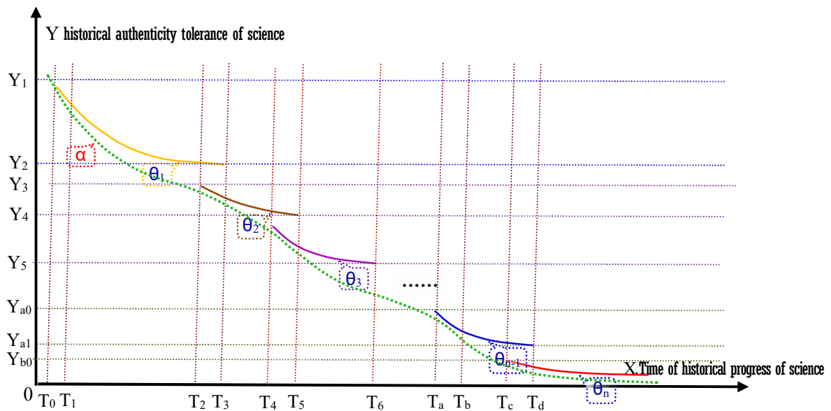
Quantitative change curve of historical progress of science making up of N successive subrogation of contemporaneous scientific Orthodoxies \Theta_1 + \Theta_2 + \Theta_3 + \dots + \Theta_{n-1} + \Theta_n in inherent optimum orientation towards perfect ideological enantiomorph of ultimate authenticity of nature
