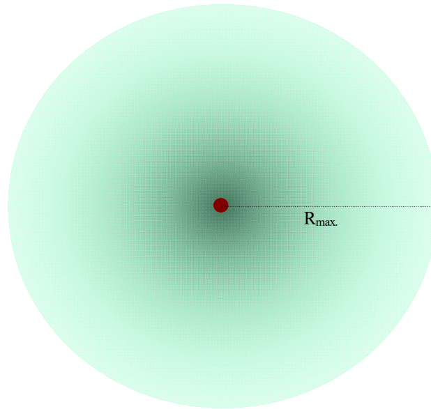
(III-i-2-a) Overall arrangement & integrated profile of positive matter and matter field
