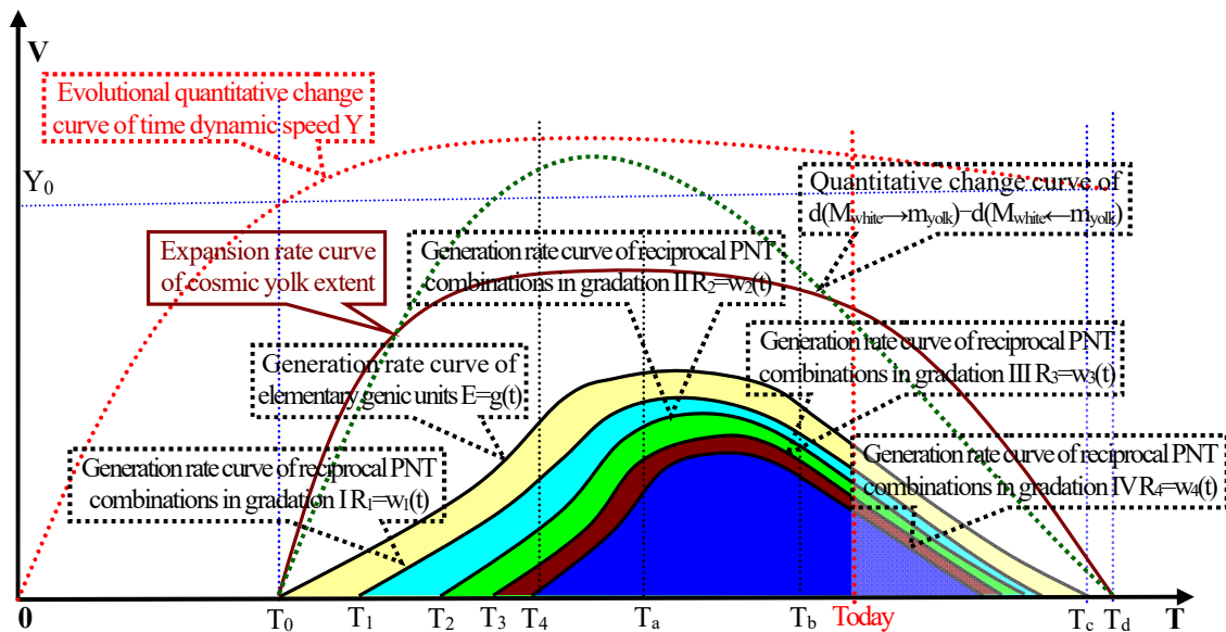
(IV-ii-5) Quantitative change rate curve of extent expansion of cosmic yolk extent, quantitative change curve of acclimatization cushion of time dynamic speed of cosmic yolk extent, quantitative change rate curve of aberrant convergence of cosmic esse due to PNT reciprocal gelation under cosmic live input of d(M_{white} \rightarrow m_{yolk}) > d(M_{white} \leftarrow m_{yolk})
