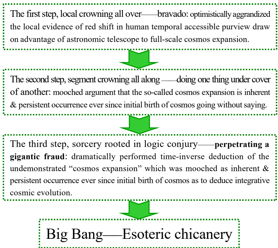
(III-ii-1) Logic extension constitution of Big Bang
