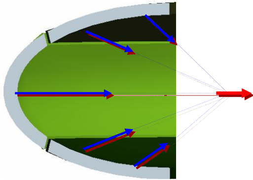
(VI-i-2~27) Section view of symmetric rectification of front PNT rectifier
