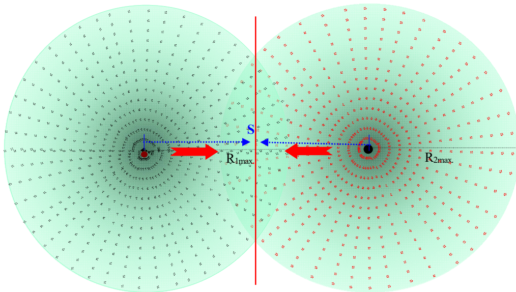
(III-i-4-c) Electromagnetic attraction between positive electric field and negative electric field
