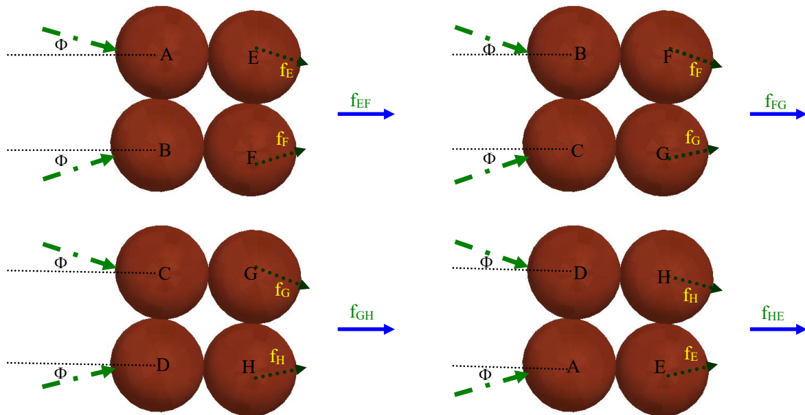
(VI-i-2~2) \Phi angle PNT activation
