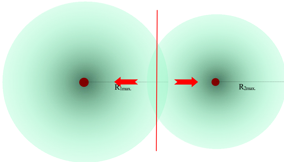
(III-i-2-c) Negative gravity due to inexpedient assimilable inadequate field superposition
