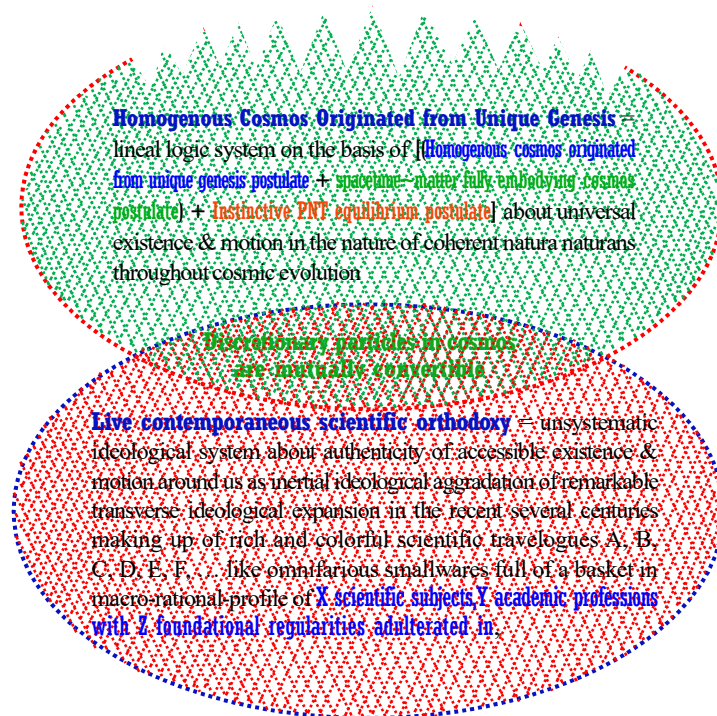
(VII-i-3) Correlation & contrast between Homogenous Cosmos Originated from Unique Genesis and Live contemporaneous scientific orthodoxy.
