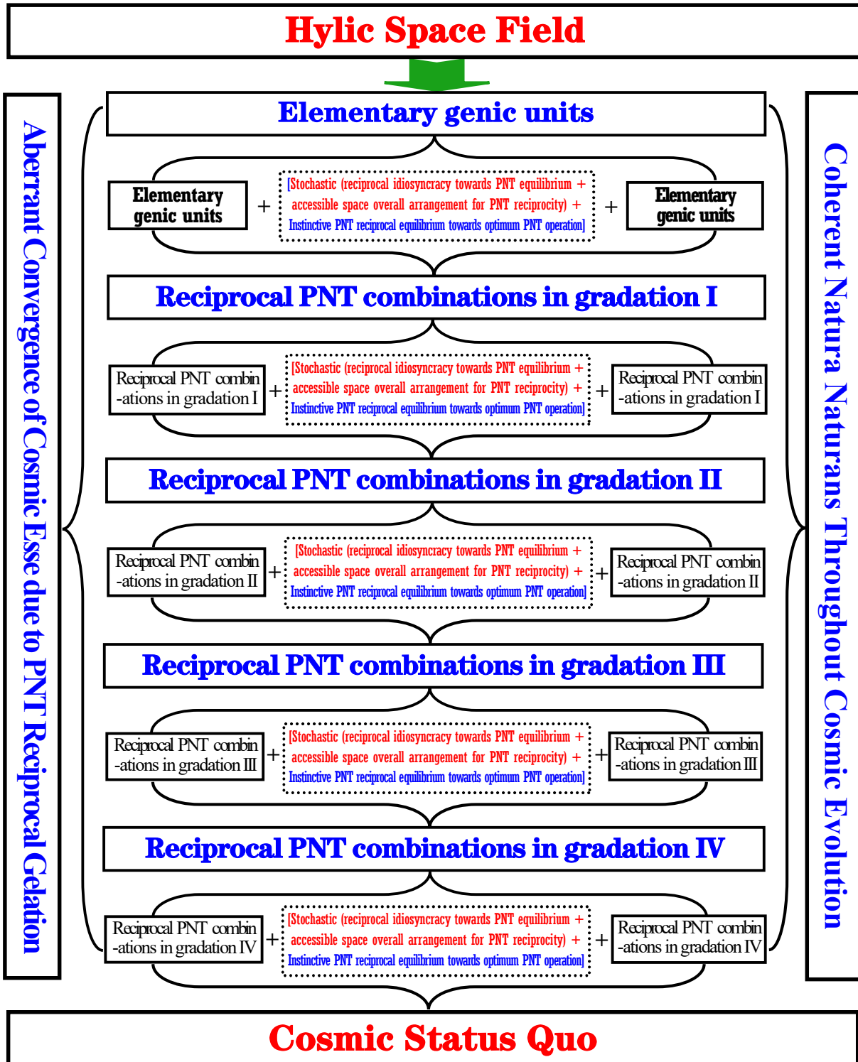
(IV-i-2) Illustration of integrative sequential homologic cosmogony
