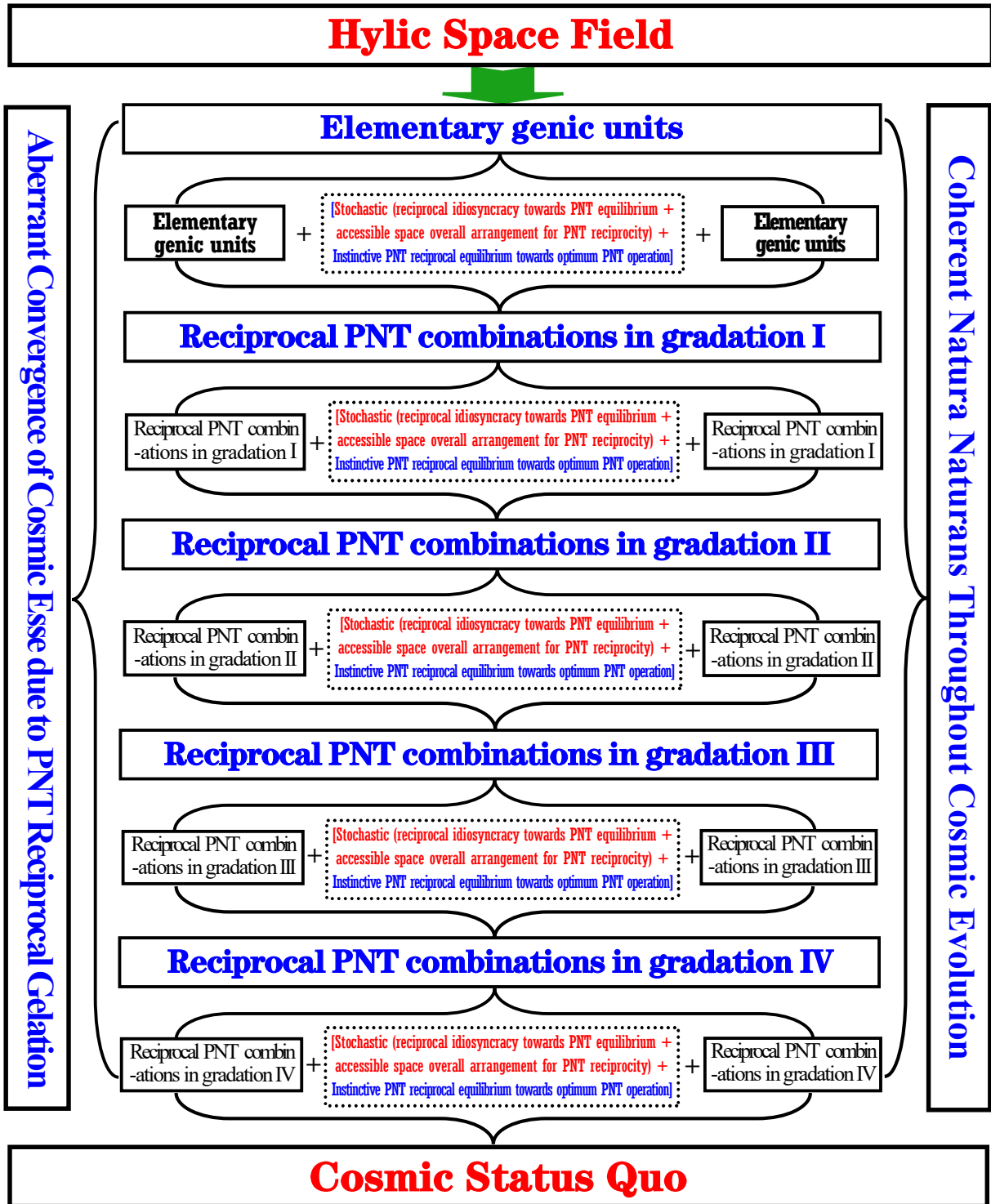
(IV-iv-5) Illustration of sequential homologic cosmogony
