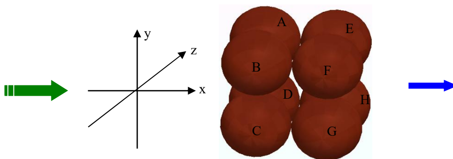
(VI-i-2~1) PNT normalized activation
