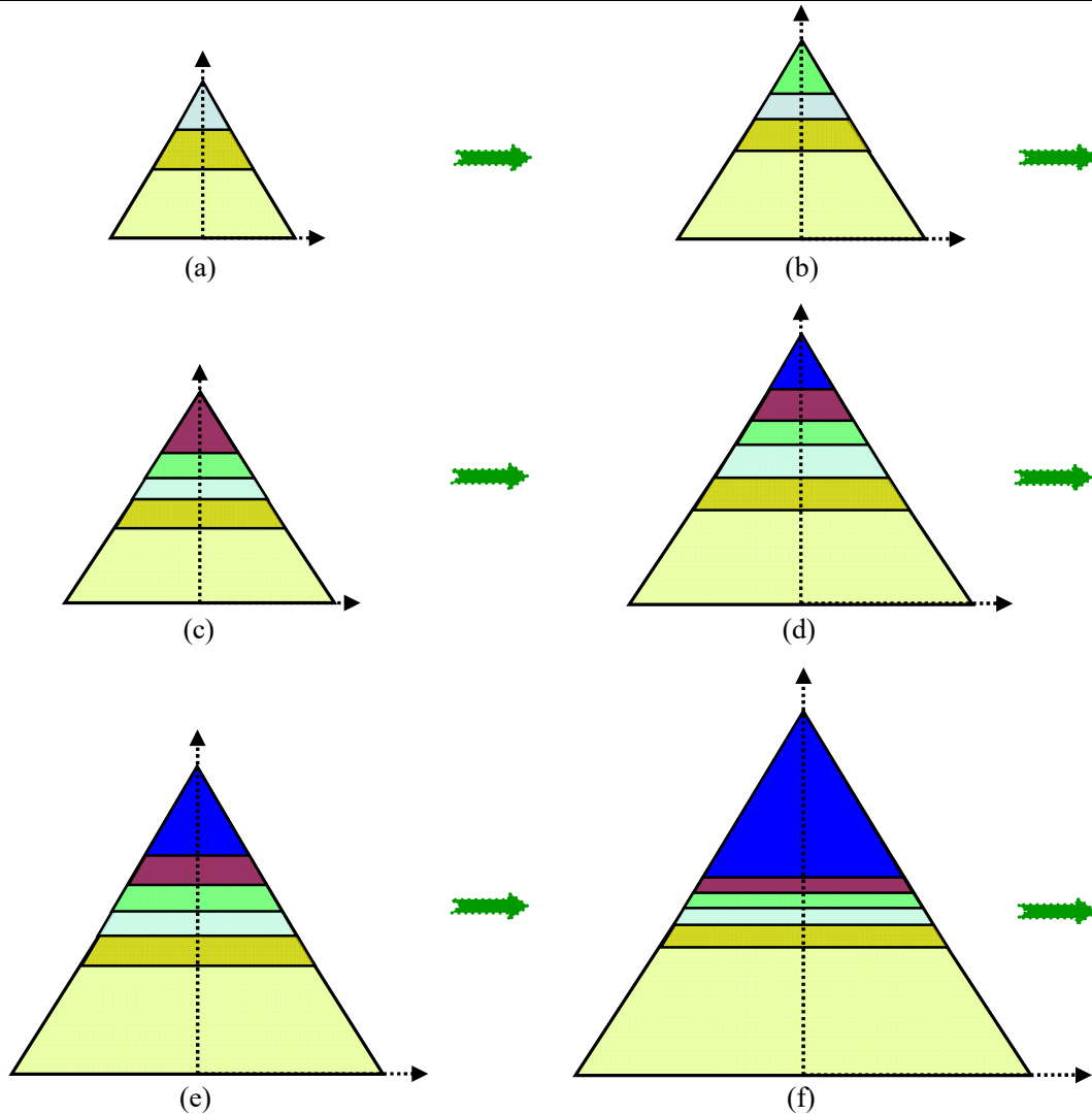
(IV-i-8) Quantitative change of the four sub phases of the third stage of cosmic evolution in expansion increase model of parallel cone
