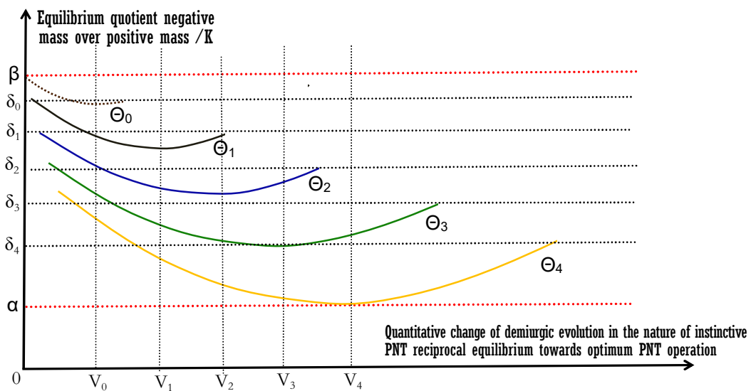
(II-i-1-b) Distribution of “equilibrium quotient negative mass over positive mass” K of matter integration along quantitative change of demiurgic evolution in the nature of instinctive PNT reciprocal equilibrium towards optimum PNT operation
