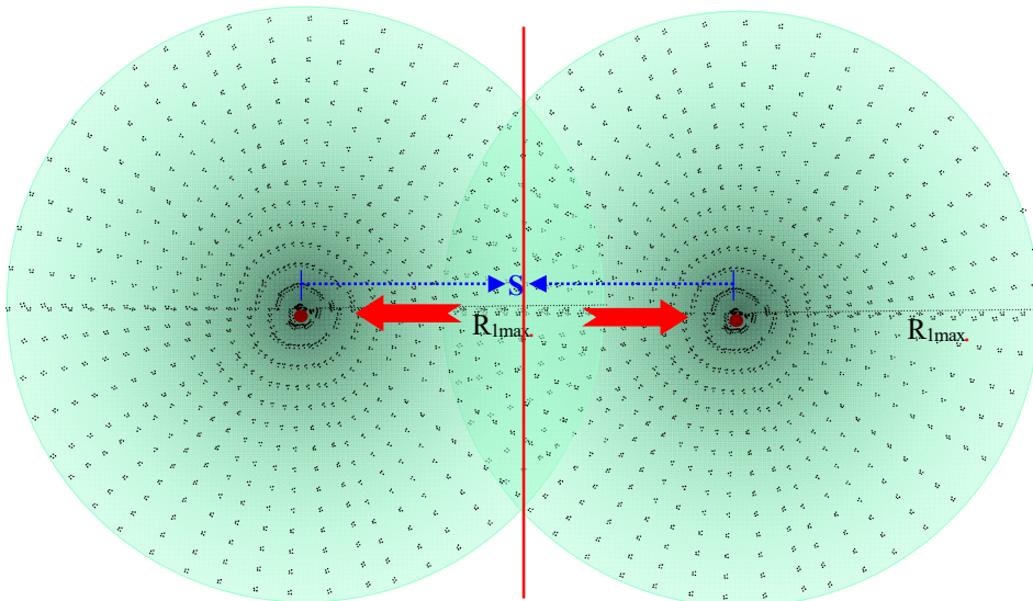
(III-i-4-d) Electromagnetic repulsion between positive electric field and positive electric field
