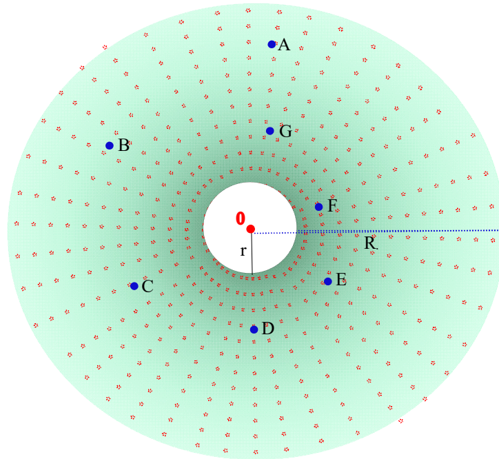
(IV-iv-2) Illustration of cosmogony in Big Bang logic model
