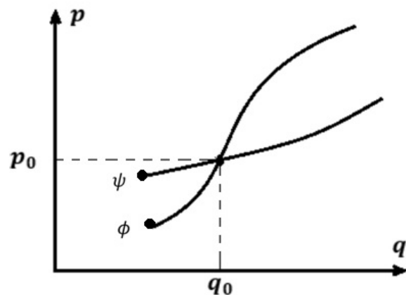
Fig. 1 The pair of initial conditions \psi and \phi , defining the distinct states of a pair of classical systems, converge at the point (q_0, p_0) , thus becoming indistinguishable. This violate the Gibbs-Liouville theorem and is therefore not allowed in classical mechanics.
