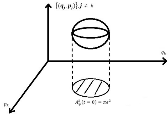
Fig. 2 The projected area A_{\psi}^k of the phase-space ball B(\epsilon) onto the conjugate pair (q_k, p_k) , at time t = 0 , is given by the minimum uncertainty area \pi\epsilon^2 .
