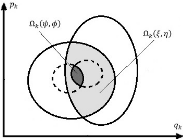
Fig. 4 Given that the overlap \Omega_k(\psi, \phi) between pairs of saturated states \psi and \phi is complex-valued, the overlap \Omega_k(\xi, \eta) between arbitrary pairs of non-saturated states \xi and \eta is also complex-valued.
