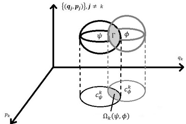
Fig. 3 Given that the state overlap \Gamma between the saturated balls B_\psi and B_\phi is complex-valued, the overlap \Omega_k(\psi, \phi) between the symplectic capacities c_\psi^k and c_\phi^k must also be complex-valued.
