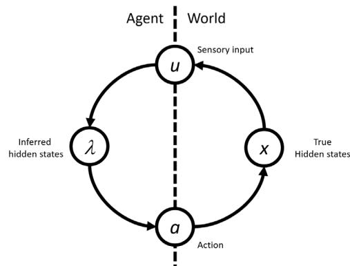
Figure 3. A simplified version of the Markov blanket shown in Fig. 1 but with depiction of circular causality induced by active inference. The dotted line marks the mind-world divide or Markov blanket; u are the sensory states of the Markov blanket, a are the active states and \lambda the internal states; x are the true hidden states of the world.
