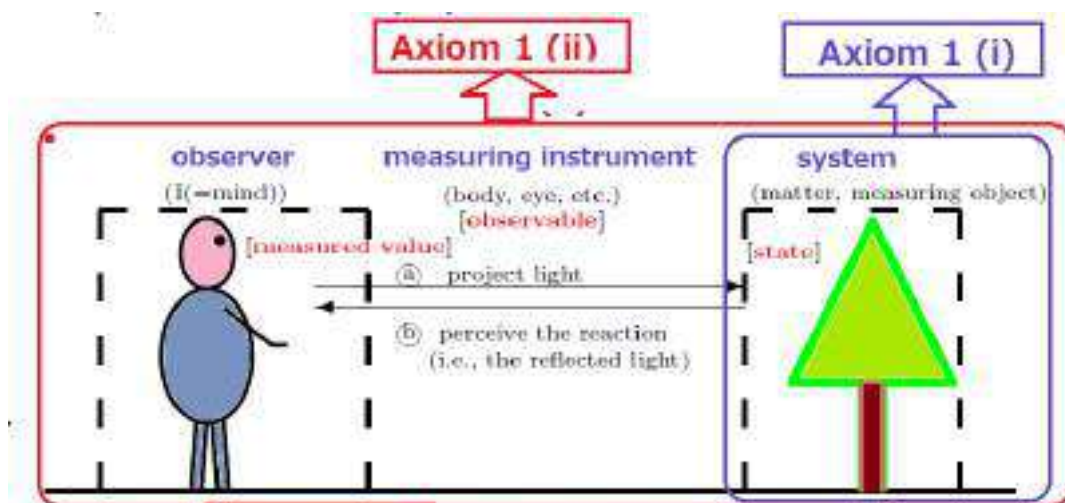
Figure 1.2. Descartes Figure: Image of "measurement(=(a)+(b))" in dualism
