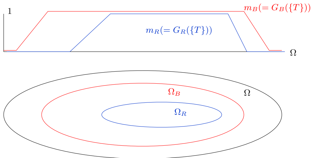
Figure 12.5, which is the same as Figure 12.4 : [All ravens are black: ( \Omega_R \subseteq \Omega_B ) ]
