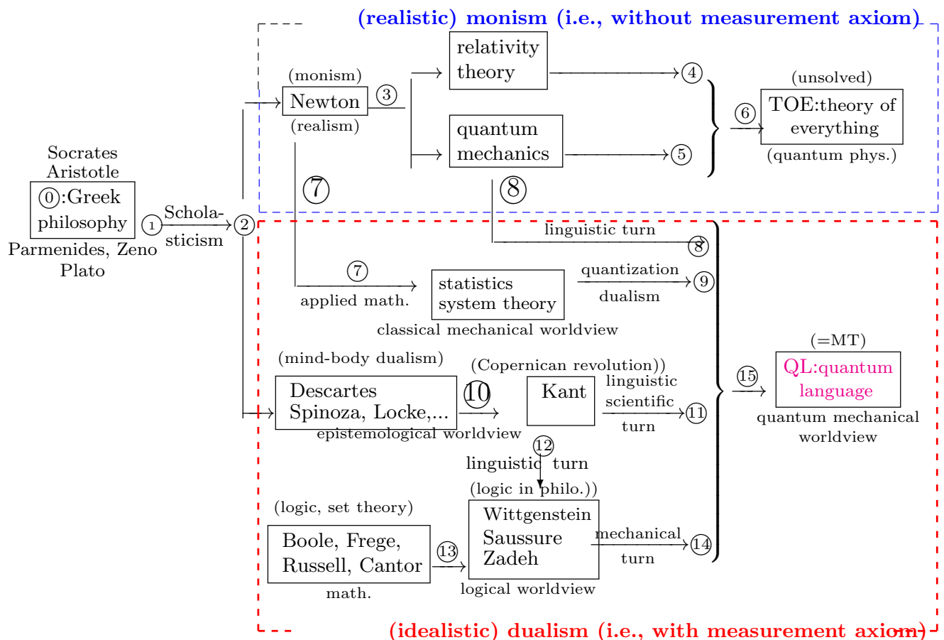
Figure 0.1 (in Preface): The history of the world-descriptions Philosophy ( \approx dualistic idealism) has progressed toward QL (i.e., ① → ② → ⑩ → ⑫ → ⑭ → ⑮)
