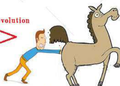
Newton
