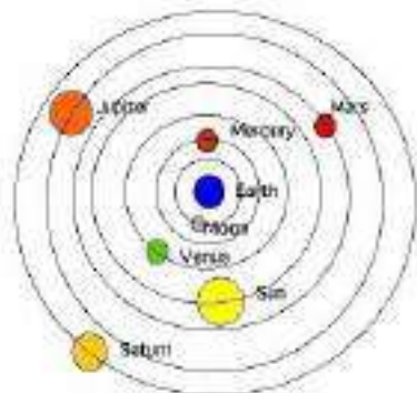
Geocentrism
