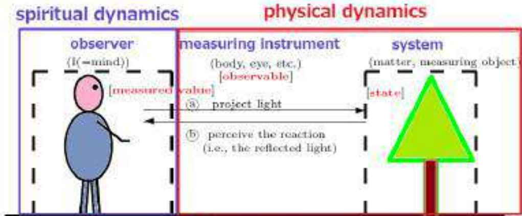
Figure 1.3. Descartes Figure : Image of "measurement(=(a)+(b))" in dualism
