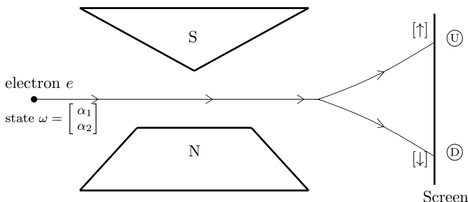
Stern–Gerlach experiment (1922)
