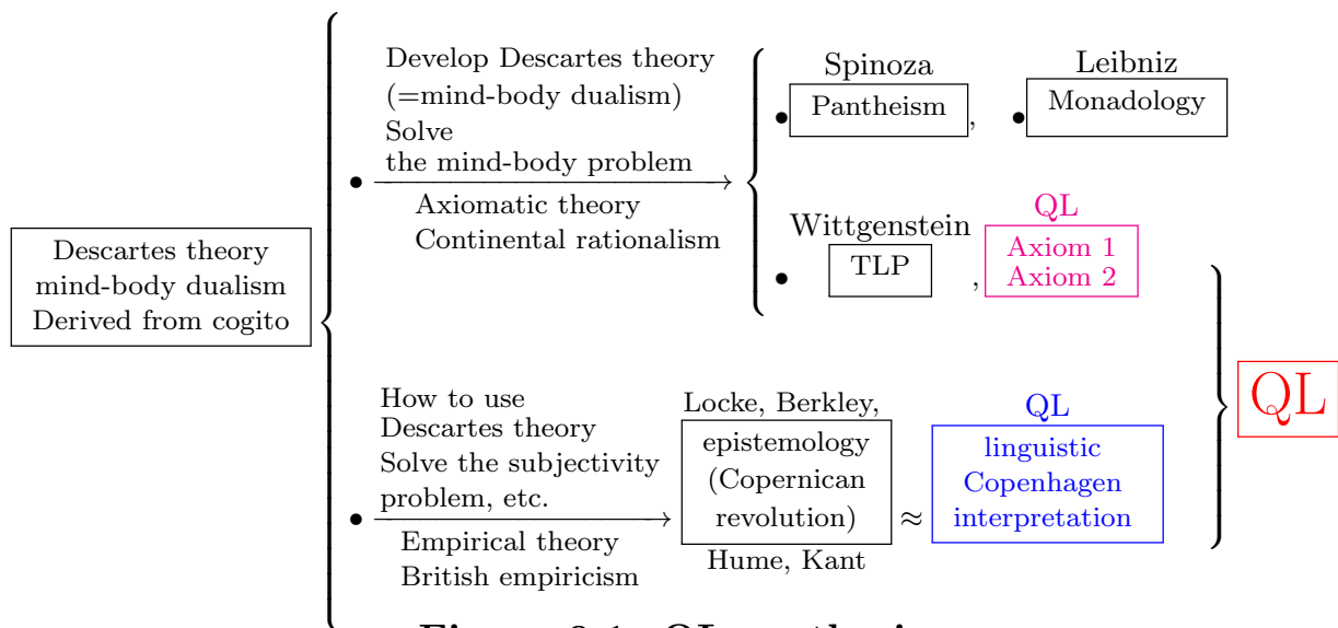
Figure 9.1: QL-synthesis
