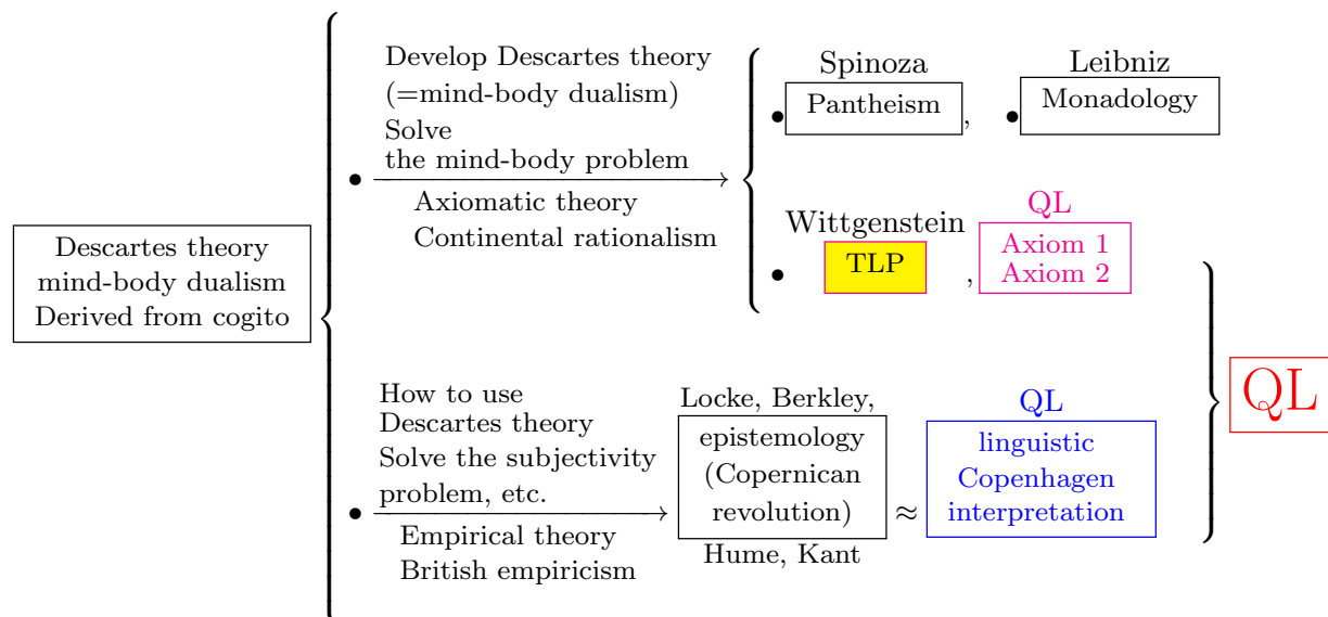
Figure 9.1: QL-synthesis
