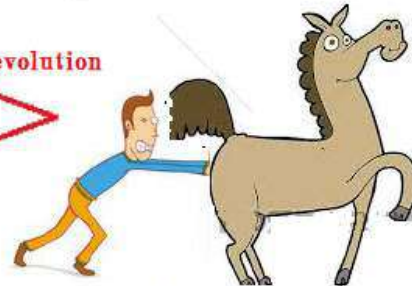
Newton
