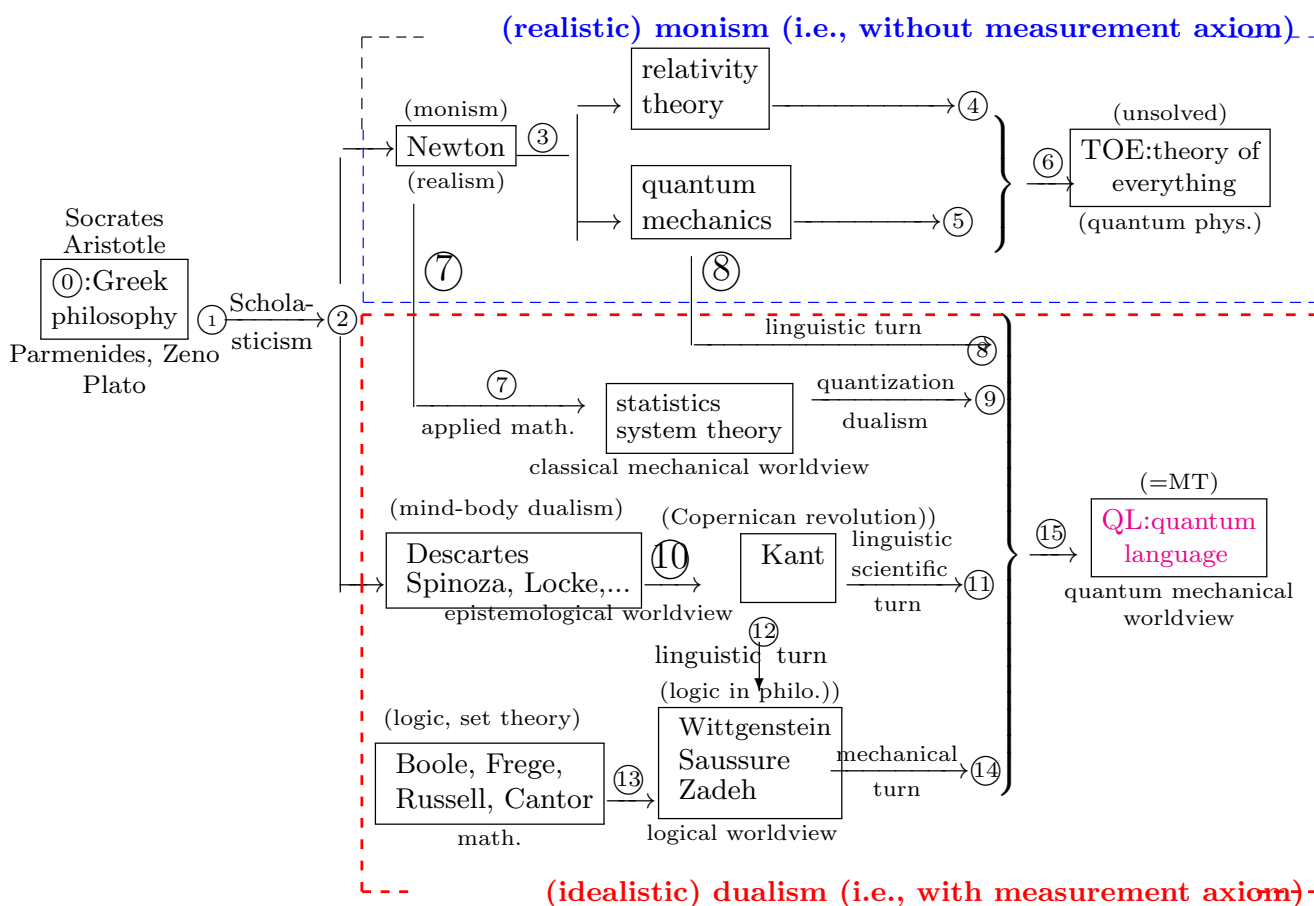
Figure 0.1 (in Preface): The history of the world-descriptions Philosophy ( \approx dualistic idealism) has progressed toward QL (i.e., 0 \rightarrow 1 \rightarrow 2 \rightarrow 10 \rightarrow 12 \rightarrow 14 \rightarrow 15 )
