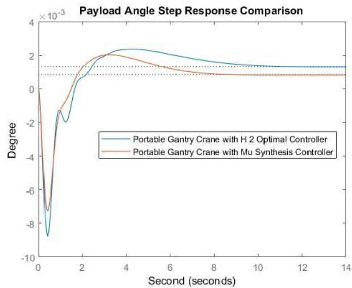
Figure 10 comparison simulation result of the step response of the payload angle
