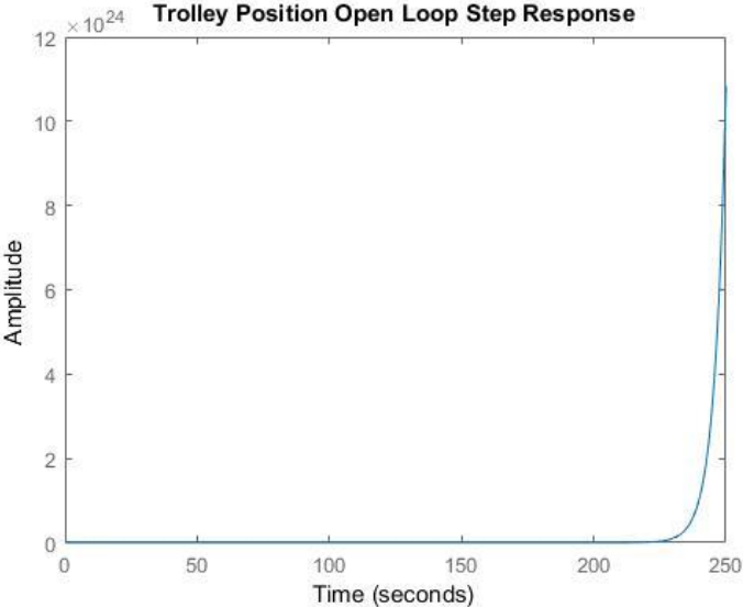
Figure 5 Trolley open loop step response
