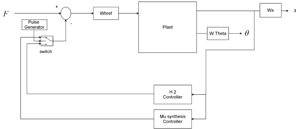
Figure 2: Portable gantry crane system with H 2 and \mu - synthesis controller's system interconnections block diagram
