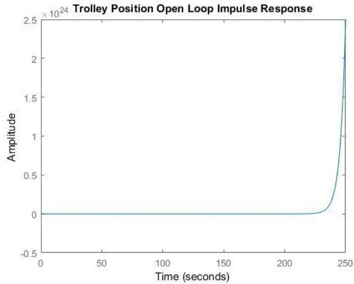
Figure 3 Trolley open loop impulse response
