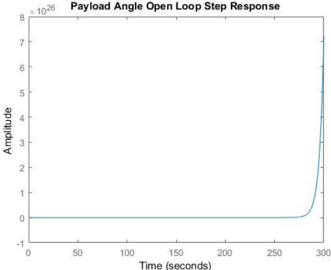
Figure 6 Payload open loop step response
