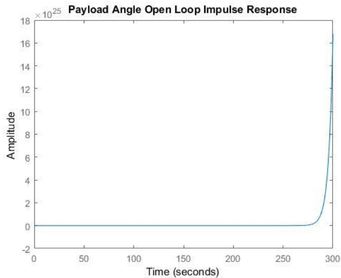
Figure 4 Payload open loop impulse response
