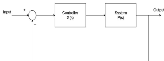
Figure 3 Block diagram of the system with H_\infty optimal control synthesis via \gamma -iteration controller
