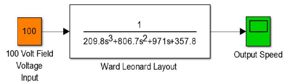
Figure 4 Simulink model of the open loop of Ward Leonard layout system
