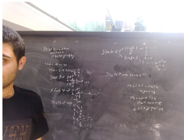
Figure 1.2: Quantum States Illustration
