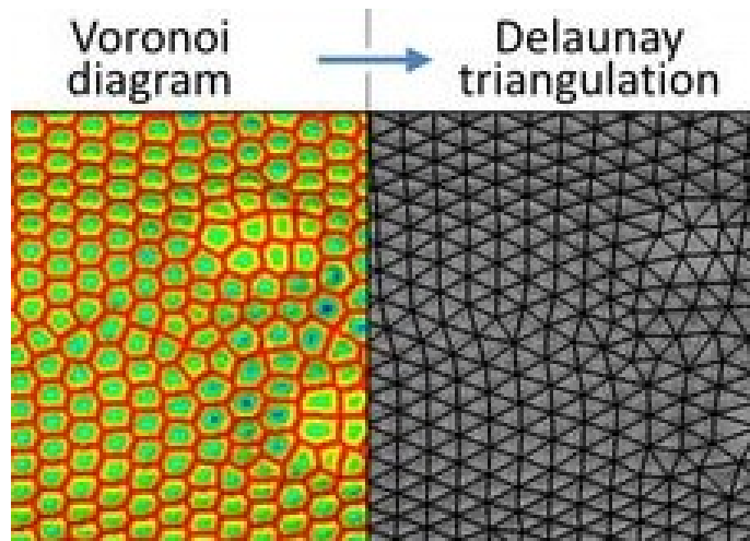
Figure 3: Voronoi tiling diagrams and Delaunay triangulation from Manukyan et al. (2017).
