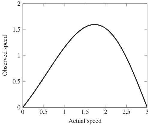
Fig. 18: Observational speed over actual speed where x = c/10^8 and the speeds are the same
