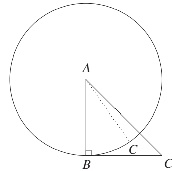
Fig. 39: The arc side
