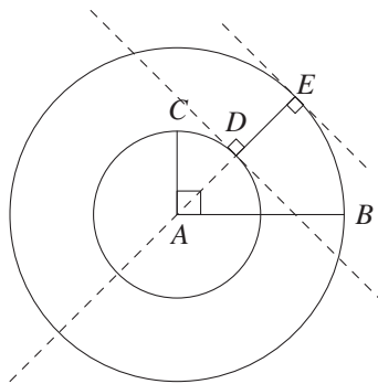
Fig. 44: The area scanned
