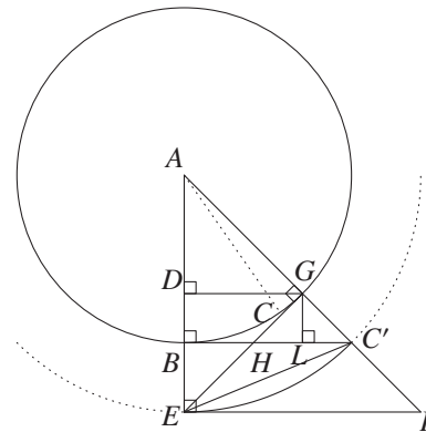
Fig. 40: The second radius
