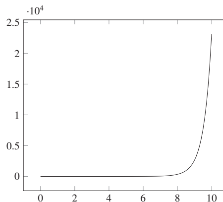
Fig. 37: Partial Palindromic prime separation
