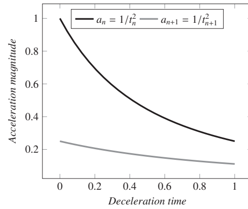
Fig. 3: Deceleration for a limited interval
