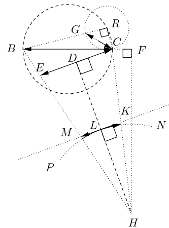
Fig. 15: Angled observation of fixed objects
