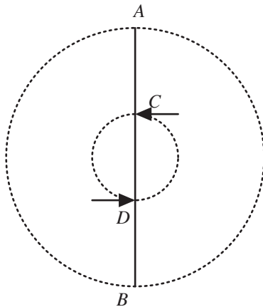
Fig. 49: An object which is about to go at light speed
