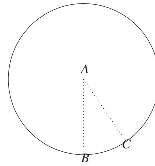
Fig. 38: Two points on the circumference
