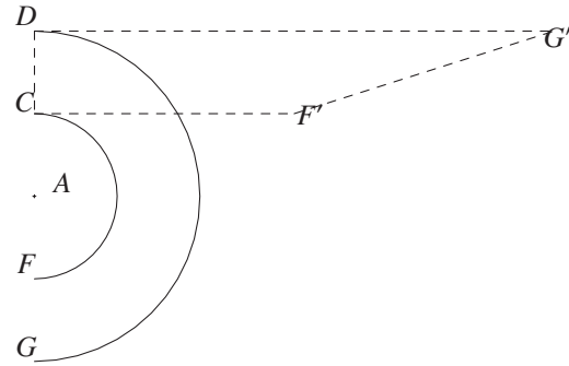
Fig. 45: The area of the circle in the kind of triangle
