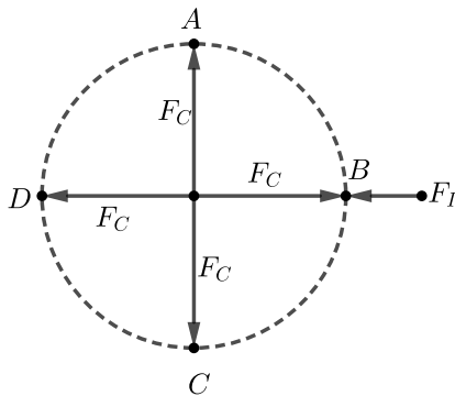
Fig. 32: Natural relativistic mass
