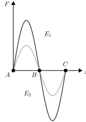
Fig. 46: Near gravitational waves
