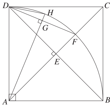
Fig. 43: The quarter slice of Fig. 42
