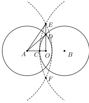
Fig. 36: Another representation of gravitational waves
