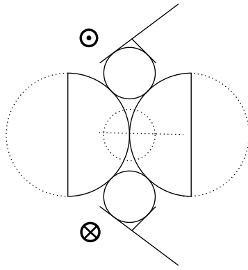
Fig. 48: The spherical balls
