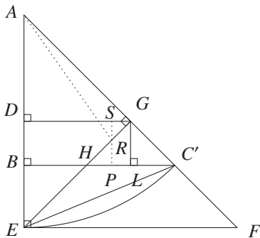
Fig. 41: A part of Fig. 40
