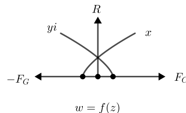
Fig. 30: Complex plane for the image set
