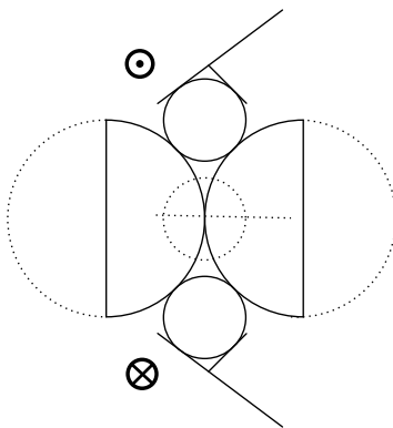
Fig. 49: The spherical balls
