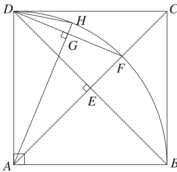
Fig. 44: The quarter slice of Fig. 43
