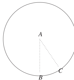
Fig. 39: Two points on the circumference
