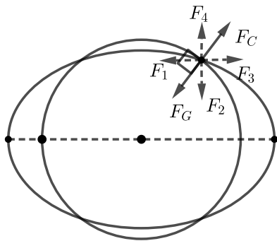
Fig. 36: Circular and elliptic orbits
