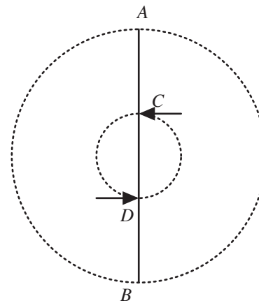
Fig. 50: An object which is about to go at light speed
