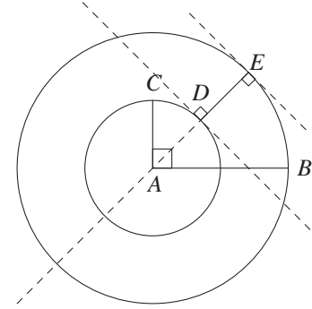
Fig. 45: The area scanned
