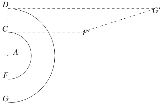
Fig. 46: The area of the circle in the kind of triangle
