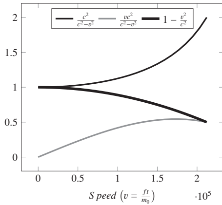
Fig. 33: Mass, length contraction and speed changing graphic from m = m_0 to m = 2m_0 , and L = L_0 to L = L_0/2
