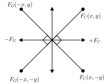
Fig. 28: Gravity and centrifugal force
