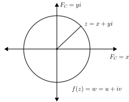
Fig. 29: Complex plane
