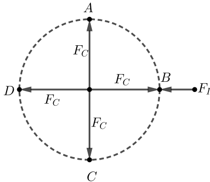
Fig. 32: Natural relativistic mass
