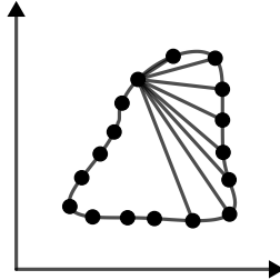
Fig. 26: Creating mass
