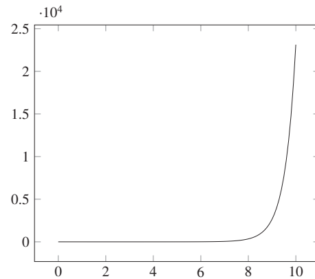
Fig. 38: Partial Palindromic prime separation
