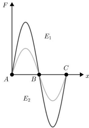
Fig. 47: Near gravitational waves
