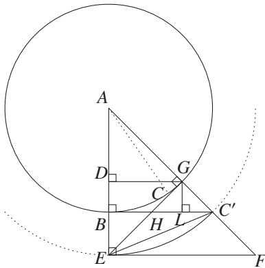
Fig. 41: The second radius
