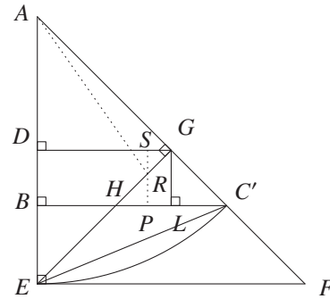
Fig. 42: A part of Fig. 41
