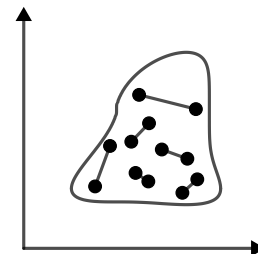
Fig. 25: Conservative area with a random closed curve
