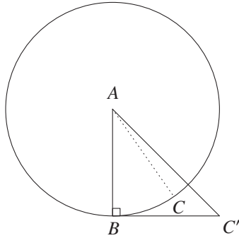
Fig. 40: The arc side
