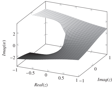
Fig. 31: Single branch of a random Riemann surface
