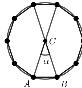
Fig. 27: Polygon transformation being n is even number
