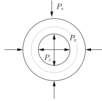
Fig. 16: Mass emergence
