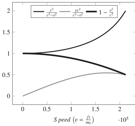
Fig. 22: Mass, length contraction and speed changing graphic from m = m_0 to m = 2m_0 , and L = L_0 to L = L_0/2
