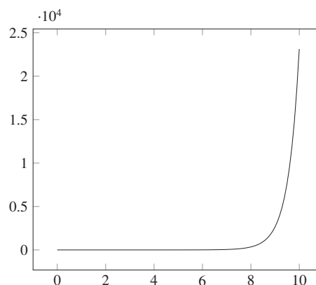
Fig. 25: Partial Palindromic prime separation
