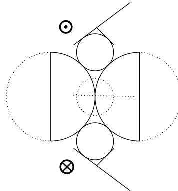
Fig. 36: The spherical balls
