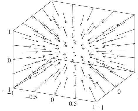
Fig. 20: Force applied for a certain mass emergence
