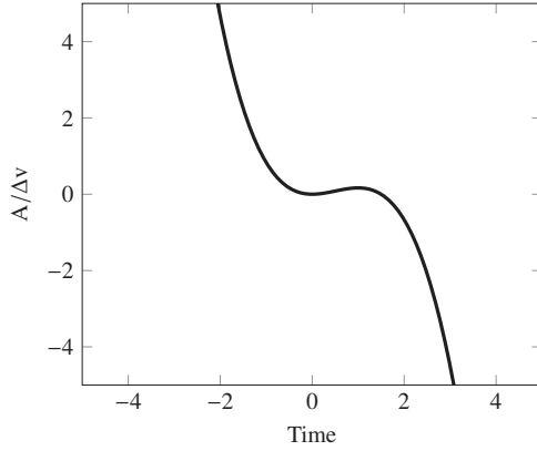
Fig. 5: A/\Delta v function
