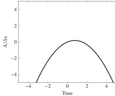
Fig. 4: A/\Delta x function
