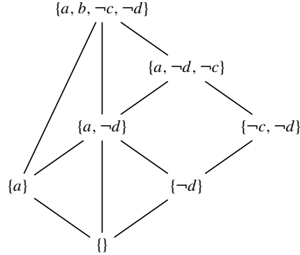
Fig. 4. Complete lattice of the strongly admissible interpretations of the ADF of Example 7.
