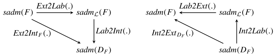
Fig. 5. The left diagram shows that strong admissibility semantics of F project to strong admissibility semantics of D_F , via Ext2Int_F . The right diagram shows that strong admissibility semantics of D_F project to strong admissibility semantics of F , via Int2Ext_{D_F} .
