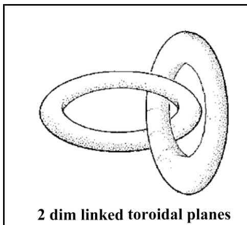
FIG.5: 2 dim linked rolled-up toroidal planes (embedded in \mathbf{R}^3 ): a first instance of potential physical complexity
