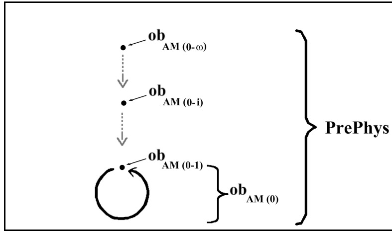
FIG.1: The tops of pre-physical emergence PrePhys : automorphic objects with a (negative ascending) strict n -categorical enrichment
