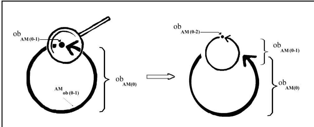
FIG.2: \mathbf{ob}_{AM(0)} , \mathbf{ob}_{AM(0-1)} and \mathbf{am}_{\mathbf{ob}_{AM(0-1)}} as seen through a magnifying glass
