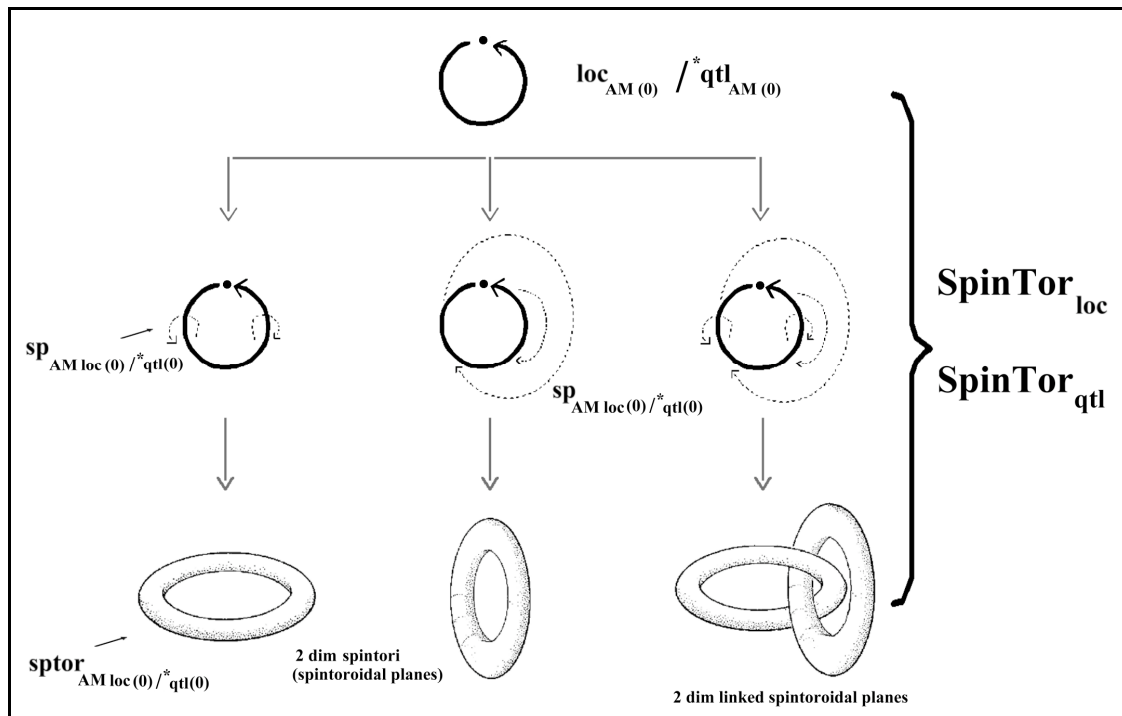
FIG.6: The topos(es) of emergence: SpinTor loc / *qtl
