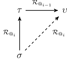
Figure 3: Upward-downward transitivity.
