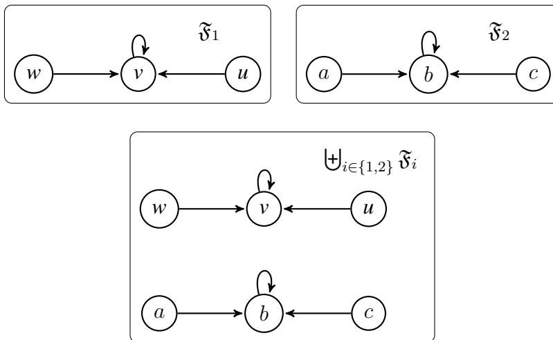
Figure 7: Non-definability of shift universality.
