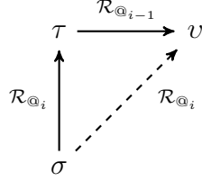
Figure 3: Upward-downward transitivity.
