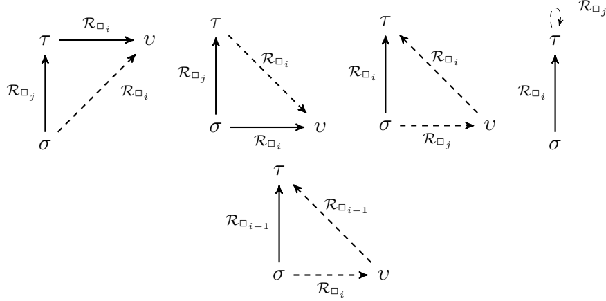
Figure 2: Upward transitivity, upward Euclideanity, downward weak density, downward shift reflexivity, and strictly decreasing weak density properties.
