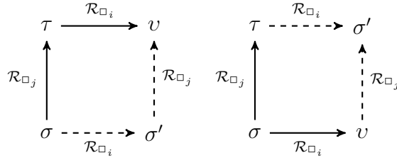
Figure 5: Left commutativity and Church-Rosser properties.
