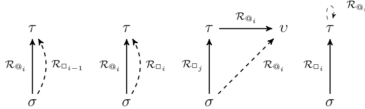
Figure 4: Strictly decreasing act-box, act-box, mixed upward transitivity, and mixed shift reflexivity properties.
