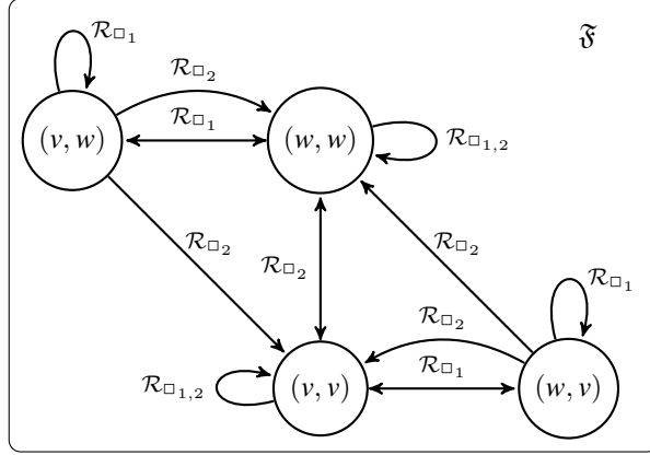
Figure 6: Two-dimensional sequence frame displaying only the \mathcal{R}_{\square_i} relations falsifying right commutativity.
