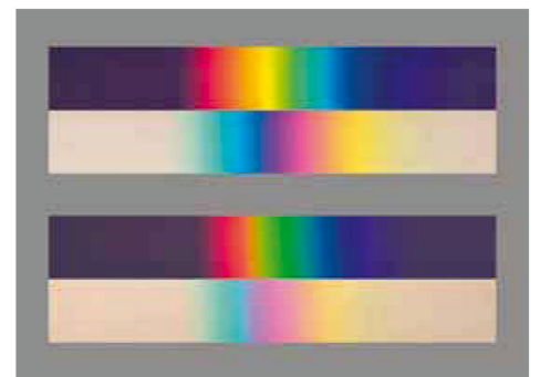
Fig 16 Two Newtonian spectra with their corresponding counterpoints [I.N. 2009]. You see a Newtonian spectrum at the top, resulting from a widely opened gap on the slide, and its complementary counterpart with exactly the same geometry. The pair of spectra at the bottom results from a comparatively narrow gap on the slide.
