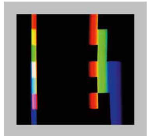
Fig 14 Nussbaumer's seven-fold colour synthesis [comparison: I.N. 2009]. If you look at the cut screen illuminated by red, green, and blue light, you see all six main colours (left). Top: red, yellow, and green – bottom: turquoise, purple, and blue. The white synthesis takes place in the middle.
