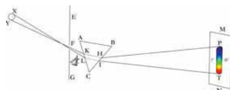
Fig 7 Desaguliers' white synthesis (1714) [redrawn with an inserted spectrum by I.N. 2009]. In Desaguliers' original drawing, two experiments are shown at once. One in which the experimenter looks at the analysis through prism AB (top), and one in which he looks through another prism CD (bottom). Newton already knew of the lower experiment. In Desaguliers, it's called "Fig. 15", which illustrates his fifth experiment; it can be found at the end of his essay (Desaguliers [AoSE]:442).
