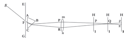
Fig 4 Newton's white synthesis (1672) [source of the drawing: Newton [NTaL]:3086; redrawn by Ingo Nussbaumer]. The multi-coloured light refracted through the prism (ABC) is collected by a convex lens (mn). Whether the white synthesis works depends on how far the screen (HI) is from the lens (mn). Some fumbling about is necessary. On the right, the figure shows three examples of screen positions that the experimenter had to try. The only optimal one is the middle position. The white synthesis only takes place there. One could say that trying to find this optimal position is like trying to find an axis of symmetry.
