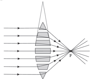
Fig 5 Lens theoretically composed of prisms [the figure is from a high-school text book, Dorn et al [PM]:238/9 (Figure 239.2), redrawn with alterations by I.N. 2009]. The figure bears the cheerful caption "convex lens composed of prism pieces", and that although it looks like prism hide-and-see, not like a clear representation of a collection of prisms.
