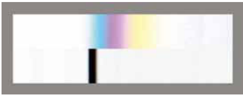
Fig 17 Nussbaumer's black synthesis [I.N. 2009]. The top of the figure shows a picture of the complementary spectrum. The bottom shows a picture of it taken by a camera through the refracting prism. All the colours of the complementary spectrum converge and mix to black.
