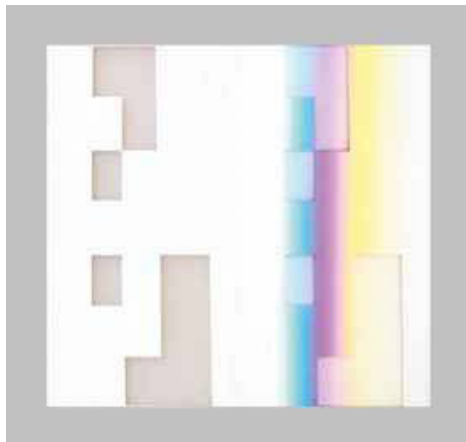
Fig 21 Nussbaumer's new pattern complementarily illuminated, [montage: I.N. 2009]. On the left, the newly cut screen (Fig.20) is illuminated from the front by a wide complementary spectrum (Fig.15) and simultaneously by equally strong white light from behind (right part of the figure). Parts of the spectrum are thereby blended out, that is, inversely cut away. This is the starting image for the sevenfold complementary colour synthesis.
