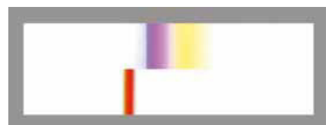
Fig 19 Nussbaumer's red synthesis [I.N. 2009]. The top of the figure shows a picture of the complementary spectrum from which the left turquoise part is removed. The bottom shows a picture of this fragmented spectrum (without turquoise) taken by a camera through the refracting prism. Purple and yellow from the complementary spectrum (all its colours except turquoise) converge and are mixed to red.
