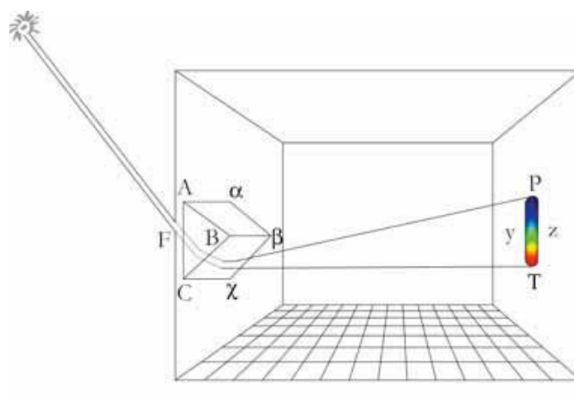
Fig 1 Newton's white analysis (1672) [colour graphic by Ingo Nussbaumer based on a drawing in Newton's sketch book; Newton's original graphic is printed in Lohne [LN]: 126/7, "Figure 1"]. Rays of light are sent through a hole in the window shutter (F) into a prism. The light is refracted and split into its multi-coloured parts.
