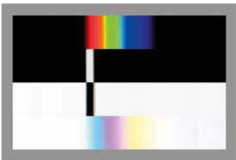
Fig. 18 Nussbaumer's white and black syntheses in synopsis [I.N. 2009]. The top of the figure shows a picture of the Newtonian spectrum (and directly below the white that results). The bottom shows a picture of the complementary spectrum (and directly above the black that results).
