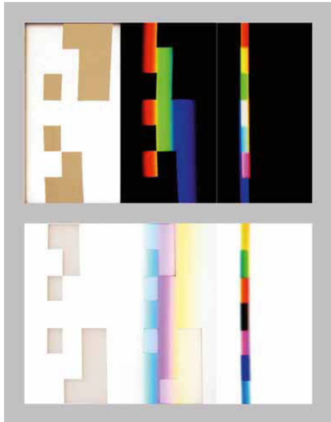
Fig 23 Comparison of both seven-fold colour syntheses [montage: I.N. 2009]. Left: each of the two slides; in the middle: the fragmented spectra as starting points (as they appear when illuminated by the spectrum); right: each of the seven-fold syntheses.
