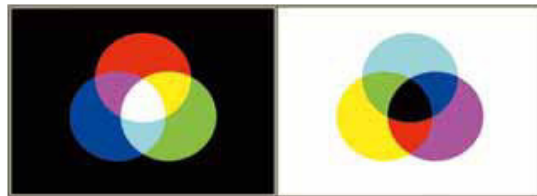
Fig 24 Two seven-fold colour syntheses [graphic: Ingo Nussbaumer [zF]: 133]. Left: the resulting syntheses from the original experiment (Fig. 13); right: their counterpoints.
