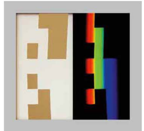
Fig 13 Nussbaumer's slide with and without spectral illumination [montage: I.N. 2009]. The cut up screen with its windows into darkness (left half) is illuminated by a wide Newtonian spectrum (right half). As both spectra have a black border along the long side, the slide only looks coloured in the middle. Here you see in each row those parts of the Newtonian spectrum that are not lost in the darkness behind the screen. One could call the image the six-fold fragmentation of the Newtonian spectrum.
