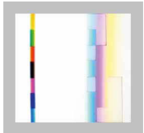
Fig 22 Nussbaumer's counterpoint to the original seven-fold colour synthesis [I.N. 2009]. If you look through a prism at the screen with its windows of brightness (right half) when it is illuminated by the complementary colours, you see again all six main colours, only in a different order. Top: yellow, green, red – bottom: purple, blue, turquoise. The black synthesis is in the middle. If you switch the top and the bottom in this picture, you get the exact complement to Fig. 14.
