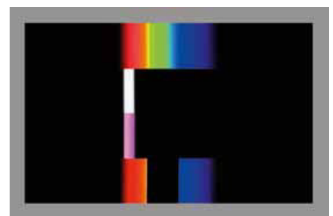
Fig 11 Comparison of the simultaneous white and purple syntheses [I.N. 2009]. The results of looking through a prism at the starting image (Fig.10) appear in the middle (rows 2 and 3). The photograph of these results proves that both syntheses are exactly the same size.
