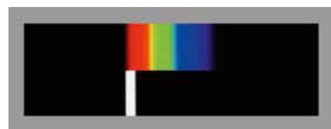
Fig 8 Photograph of the Viennese white synthesis [I.N. 2009]. The top of the figure shows a picture of the Newtonian spectrum. The bottom shows a picture of it taken by the camera through the refracting prism. All the colours of the Newtonian spectrum converge and mix into white.
