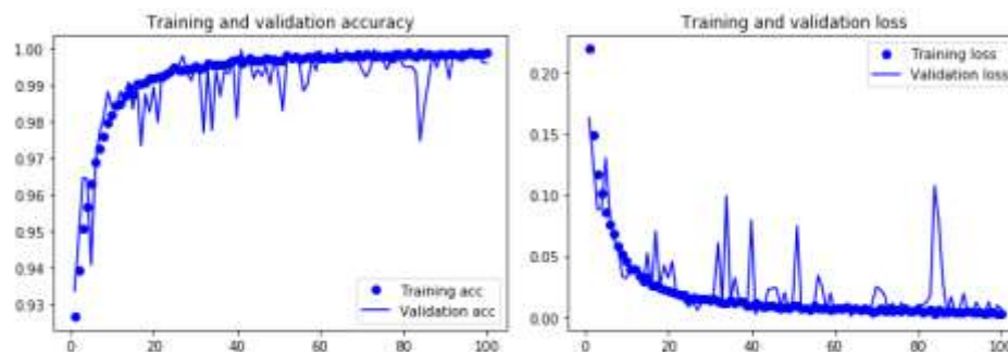
Figure 4: Training and validation accuracy and loss
