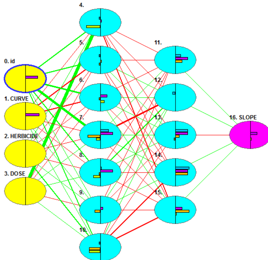
Figure 1: Shows the Design of the Neural Networks
