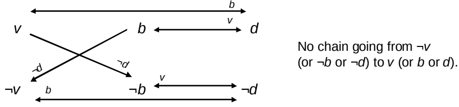
Figure 2: The agenda \overline{\overline{X}} violates (b).
