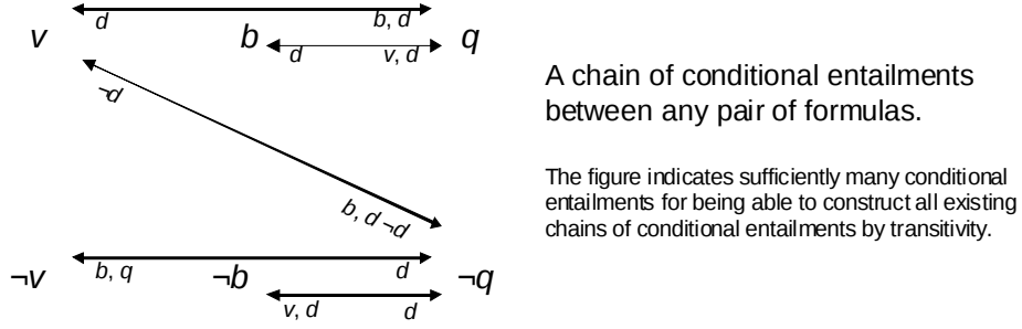
Figure 4: The agenda \overline{X} with P = \{b, v, q\}^\pm satisfies (b_P) .
