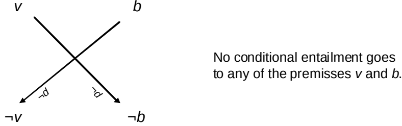
Figure 5: The agenda \overline{\overline{X}} with P = \{b, v\}^\pm violates (b_P) .
