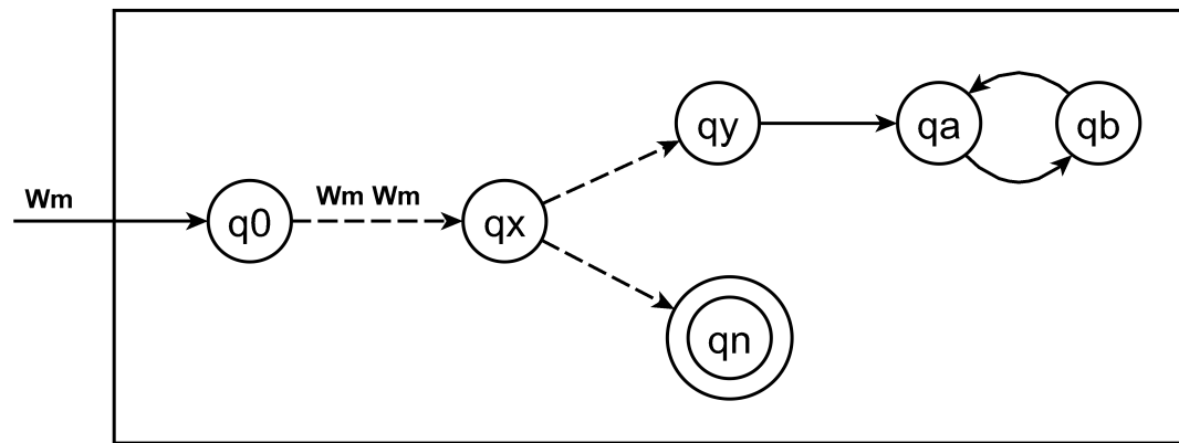
Figure 12.3 Turing Machine \hat{H}
