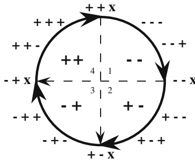
Figure 4. The crossed circle as a 12CR map.
