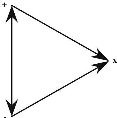
Figure 2. The triangle as a ILSR map.
