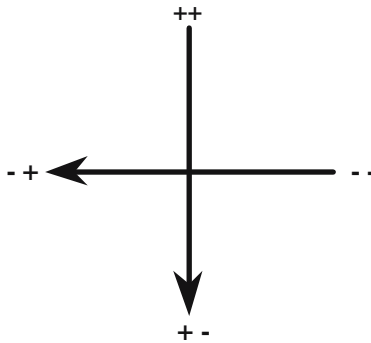
Figure 3. The cross as a 2LAR map.
