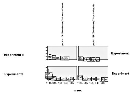
Fig. 18. The statistically significant contrast in the variability of intrinsic mode functions between the two experiments correlated with a contrast in access is for the instantaneous amplitude within the 2 variables postIMF 7 DiamondPseudo and postIMF 7 SquarePseudo (T5).
