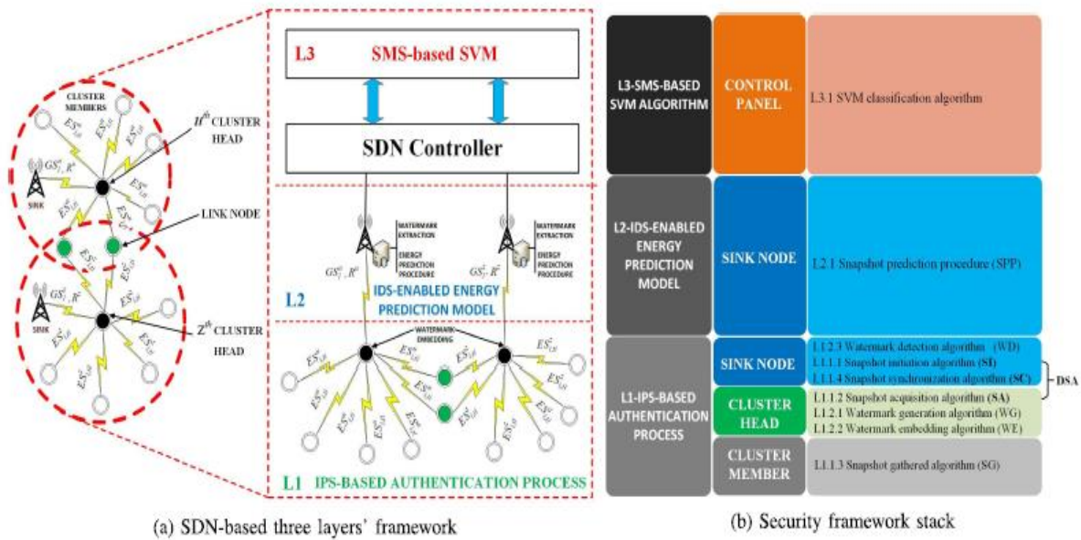
Figure 1. SDN Based Three layer and Security Framework Stack
