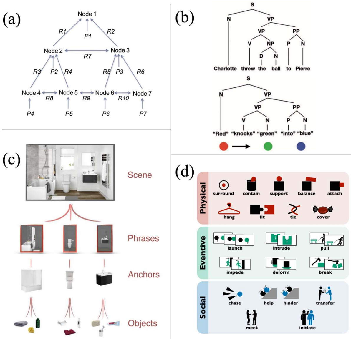
Figure 3. (a) Hierarchical part-whole structural description: Ps=monadic featural properties, horizontal Rs=spatial relations, vertical Rs=mereological relations; reprinted from Green (2019),
