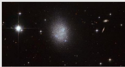
A dwarf galaxy. Image Credit: NASA/ESA
