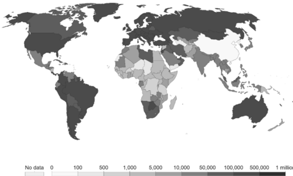
Figure 1: Global map confirm COVID-19 cases per million people (February 22 nd , 2022)
