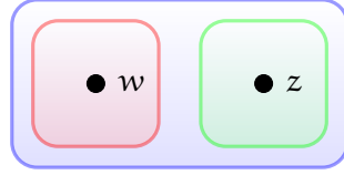
Figure 3: A = \{v_1, v_2, v_A\} , \mathbb{E}(w) = \{\{w\}, \{z\}, W\}
