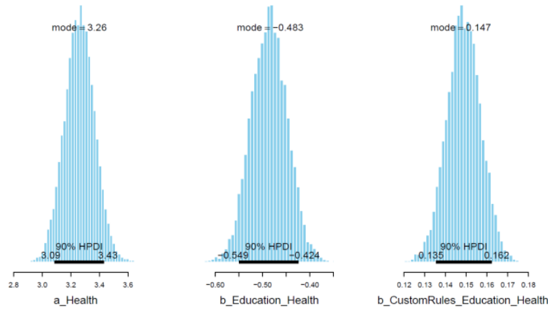
Figure 3. Posterior coefficients distributions
