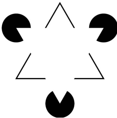
Figure 1: Kanizsa Triangle
