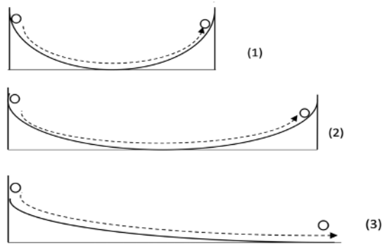
Galileo's Thought Experiment on Inertia
