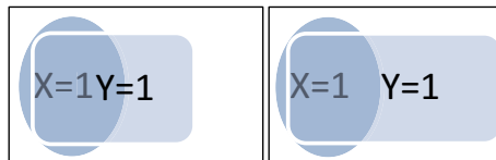
Fig. 2. Venn diagrams illustrating the MT alternative antecedent prediction.
