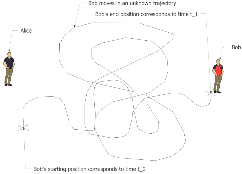
Figure 13: Alice is calculating Bob's relative velocity, while Bob moves with an unknown trajectory.
