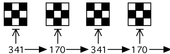
Figure 4. A short thought-stream supports a cellular automaton.
